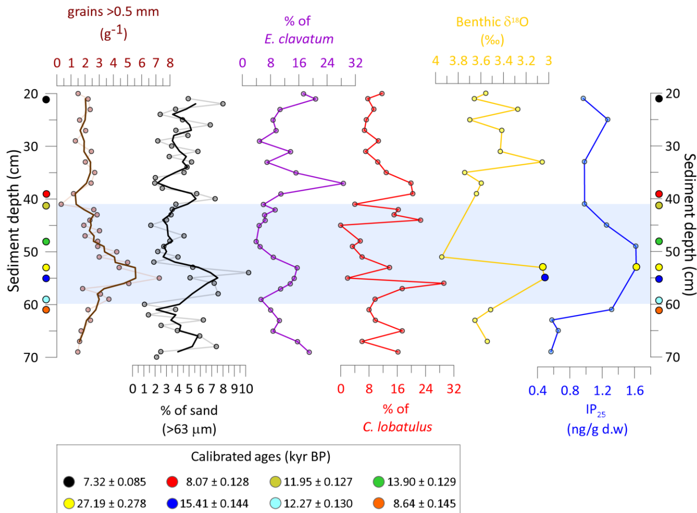
Supplementary Figure 1. | Combined records of bulk parameters, foraminiferal, stable oxygen isotope, and sea ice proxy from core KV02. From left to right: Concentrations of grains >0.5 mm, percentage of sand (>63 μm), percentage of Elphidium clavatum , percentage of Cibicides lobatulus , benthic foraminiferal δ 18 O, and IP 25 concentrations. Light blue shading indicates a redeposited layer. Symbols next to the left and right y-axes indicate AMS 14 C dates.
