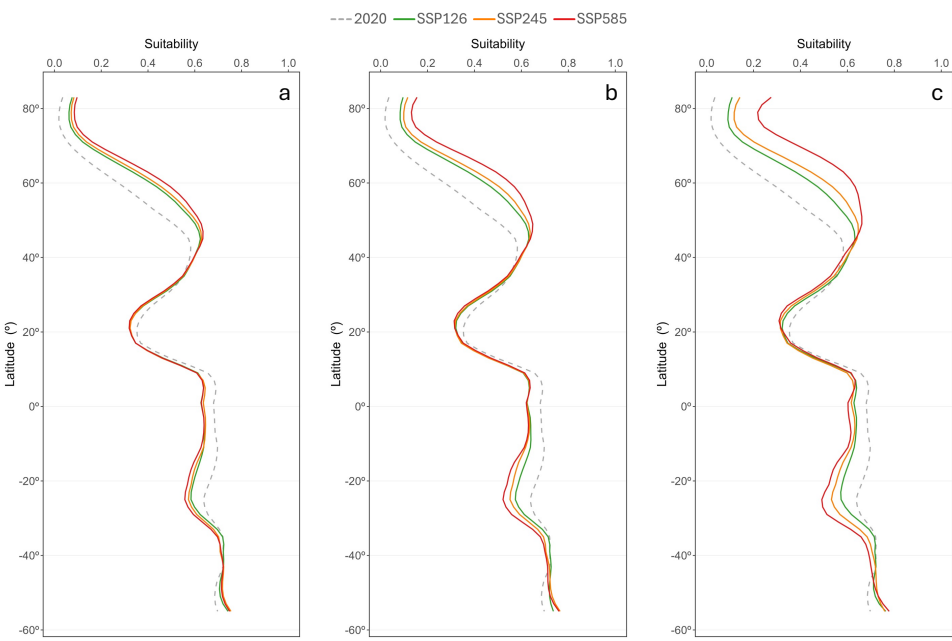
Fig. #. Mean logistic output (probability of presence) according to latitude for A. fumigatus under current and future climate modelling scenarios for various SSPs. Future time horizons: (a) 2041-2060, (b) 2061-2080, (c) 2081-2100.
