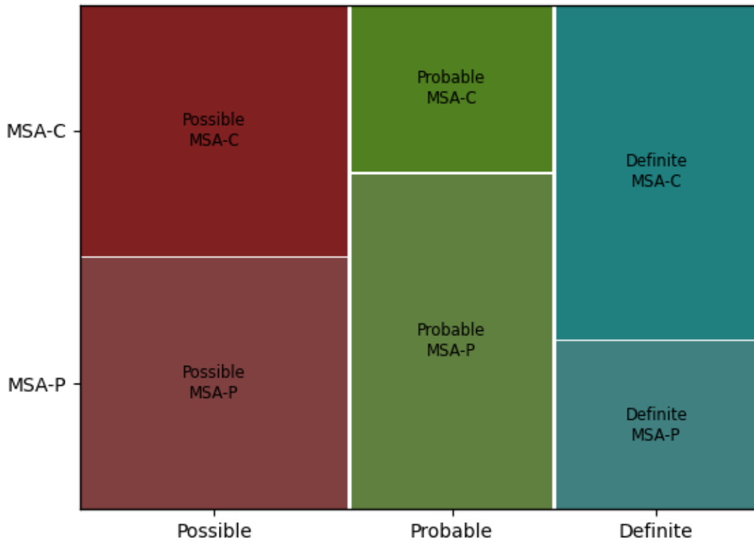
Mosaic Plot of MSA Classification and Clinical Diagnosis
