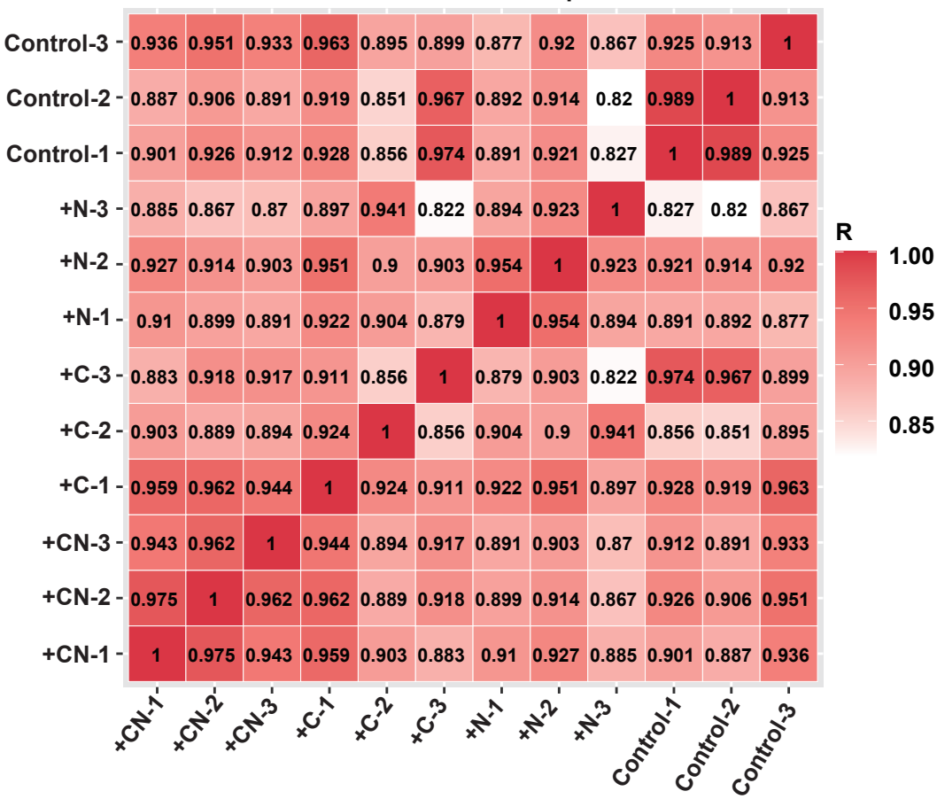
Correlation Heatmap
