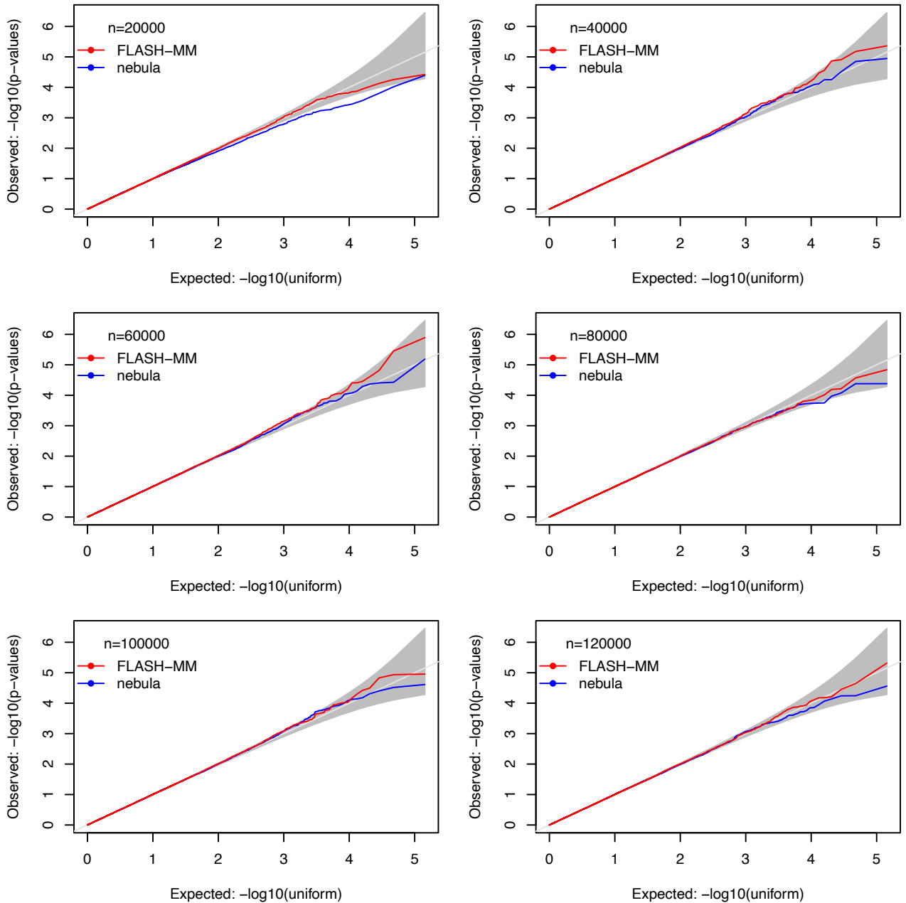
Extended Figure 1) QQ-plots of FLASH-MM and nebula p-values. QQ-plots of FLASH-MM and nebula p-values under the null hypothesis H_0 in different sample sizes n .
