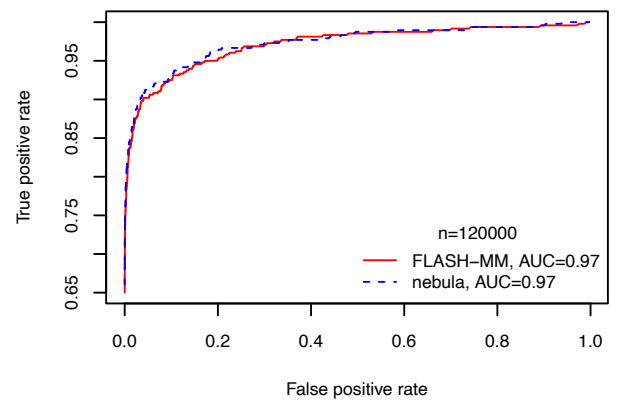
Extended Figure 2) ROC curves of TPR versus FPR for FLASH-MM and nebula in different sample sizes ( n ).
