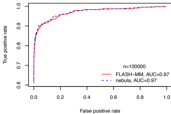
Extended Figure 2) ROC curves of TPR versus FPR for FLASH-MM and nebula in different sample sizes ( n ).
