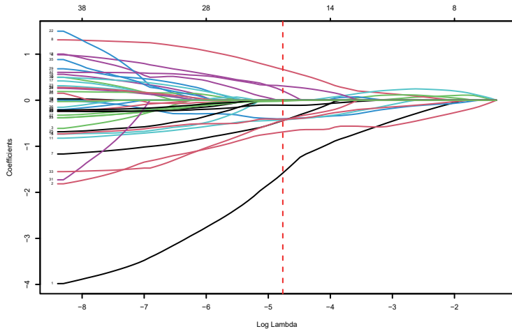
Coefficient Paths for Elastic Net Regression
