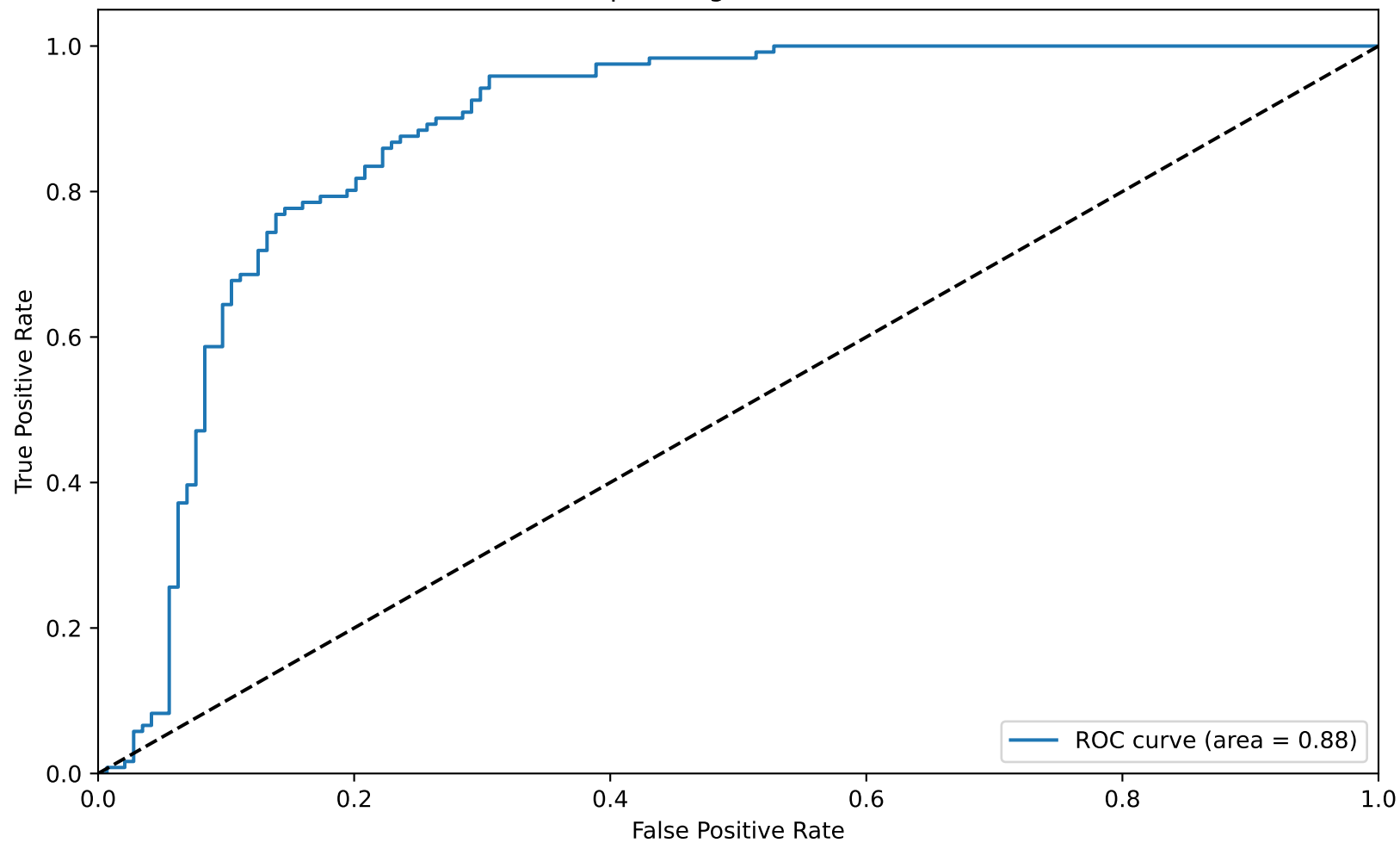
Receiver Operating Characteristic (ROC)
