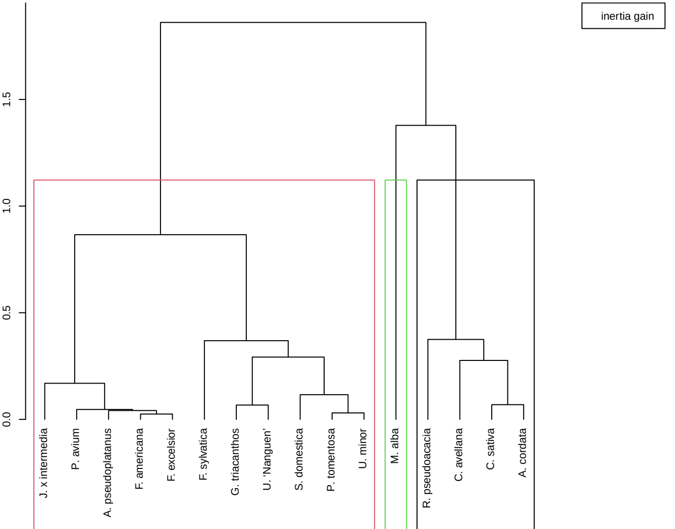
SM 3 Dendrogram of the hierarchical clustering on principal components
