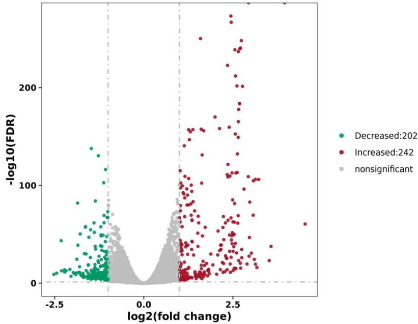
Supplemental Figure 1. Volcano plot of differentially expressed genes between the LSDV infection group and the \Delta Orf132 infection group
