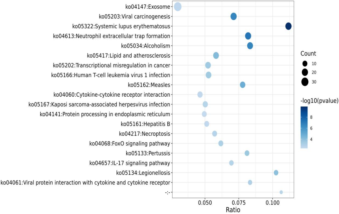
Supplemental Figure 3. KEGG enrichment analysis of differential genes between the LSDV infection group and the LSDV- \Delta Orf132 infection group
