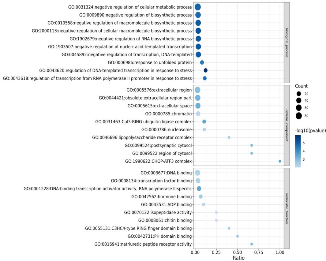
Supplemental Figure 2. GO enrichment analysis of differential genes between the LSDV infection group and the LSDV- \Delta Orf132 infection group
