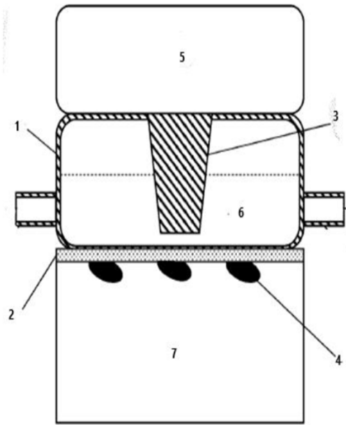
Figure 1: Feeding Device
