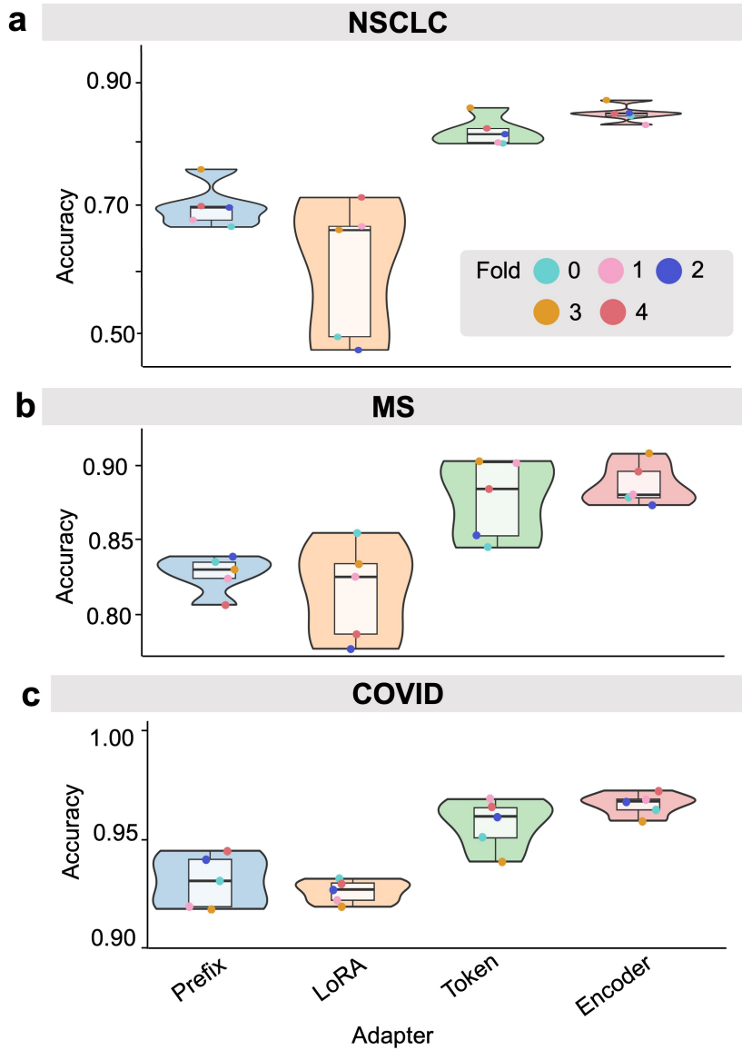
Supplementary Figure 1. Violin plots of diverse adapters in scPEFT across multiple datasets. These violin plots showcase the performance of diverse adapters in scPEFT with the scGPT backbone for cell type identification across (a) NSCLC, (b) MS, and (c) COVID datasets respectively.
