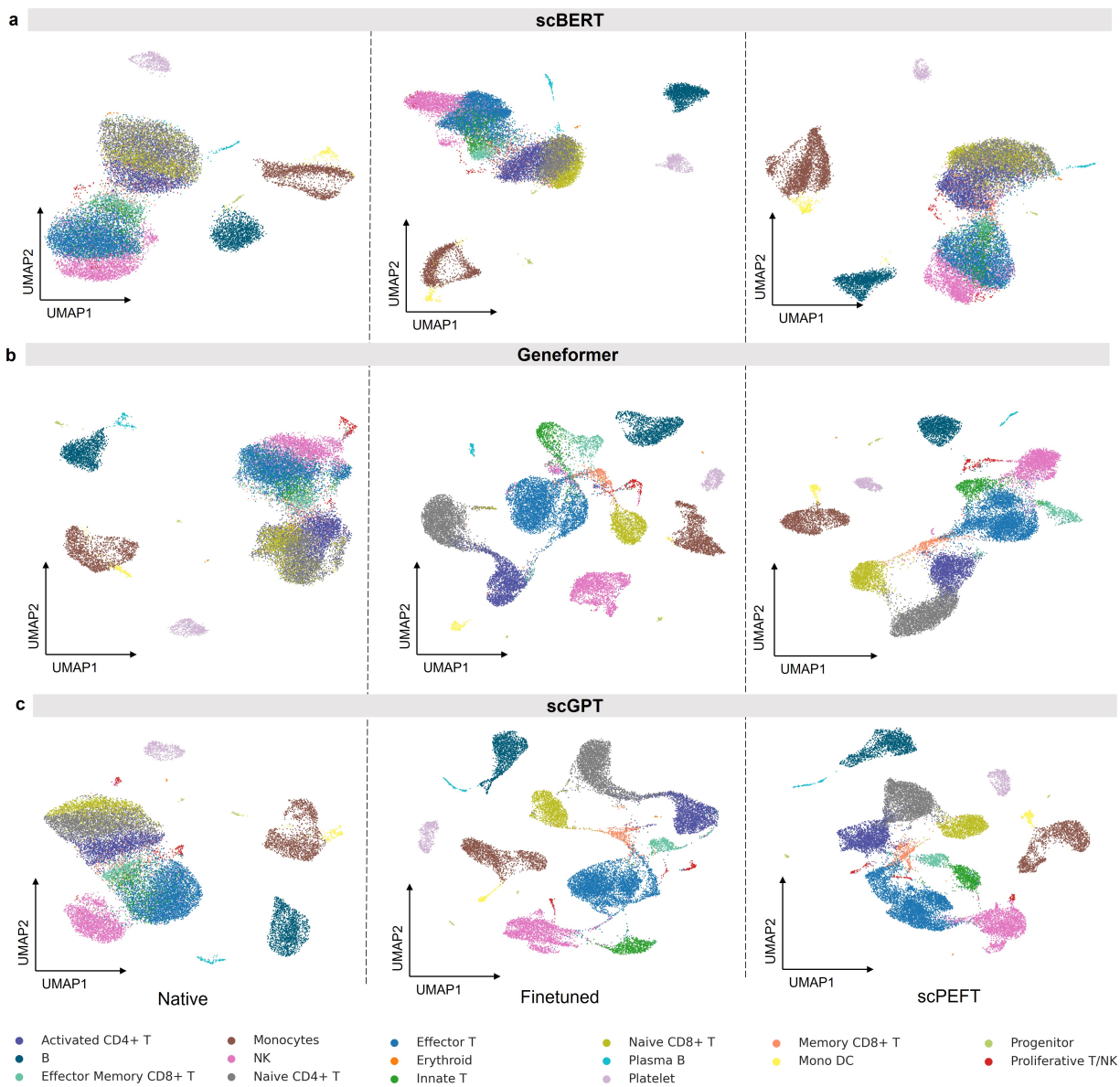
Supplementary Figure 4. UMAP visualizations of cell type identification on the COVID dataset. The UMAP visualizations were generated from the native, fine-tuned scLLMs, and scPEFT models with different backbones (a) scBERT, (b) Geneformer, and (c) scGPT, respectively.
