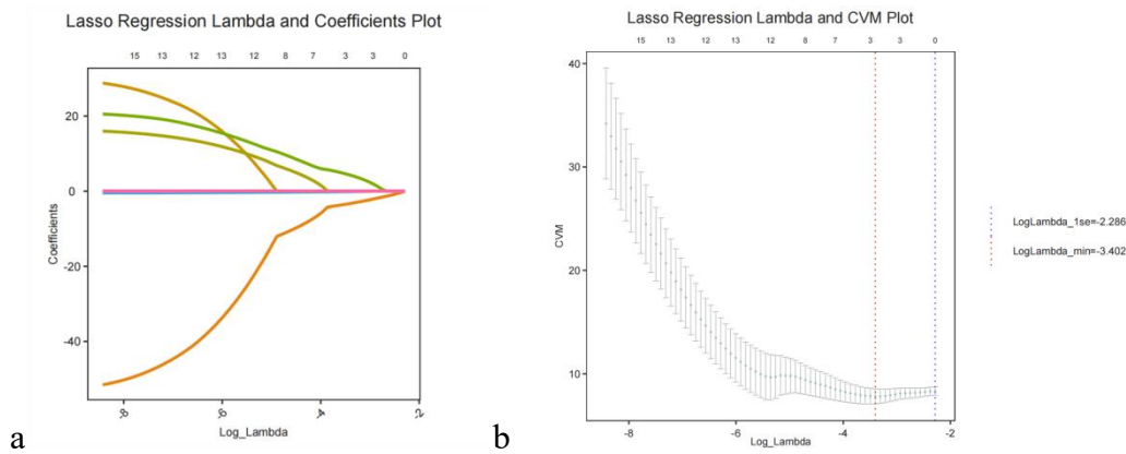
Supplementary FIG.1 (a) Least absolute shrinkage and selection operator (LASSO) coefficient profiles of model via penalized maximum likelihood with L1 - norm regularization. (b) Hyperparameter of the LASSO regression model was performed by 10 - fold cross - validation method. Use the minimum standard (left dotted line) and 1 - standard error (SE) criteria (right dotted line) to draw a vertical dashed line at the optimal value. The optimal lambda produced three nonzero coefficients.
