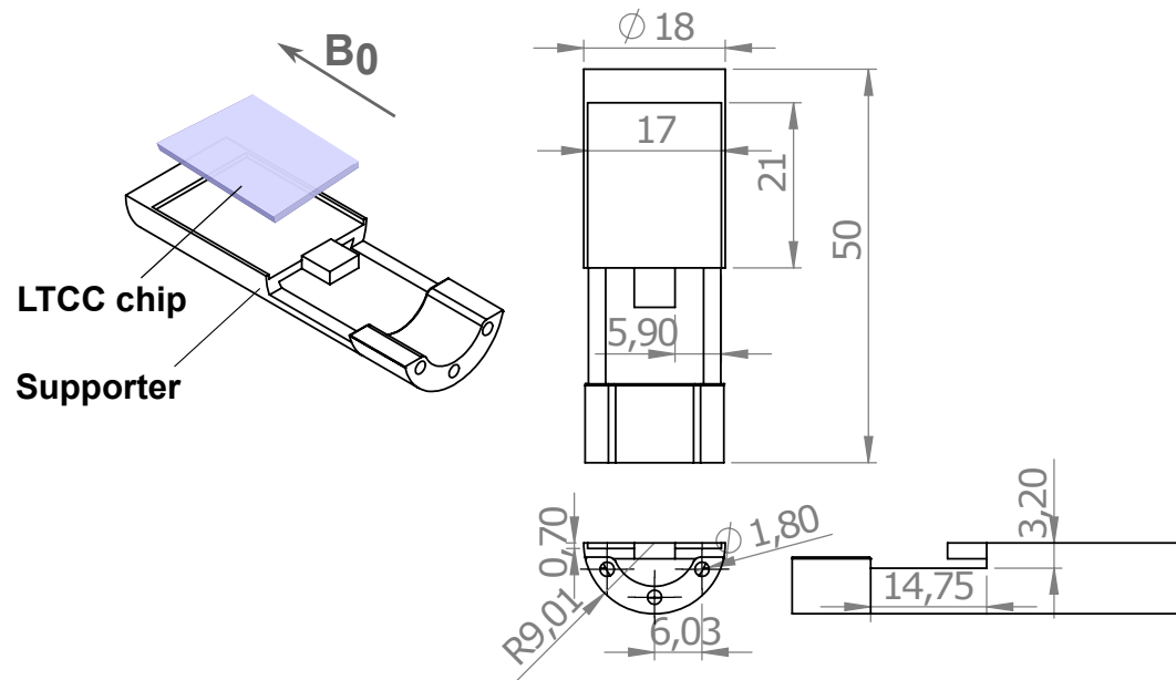
Figure S1: Assembly of the chip model with SLA 3D printed supporter. The dimensional parameters are shown in 3 views in the unit of mm.
