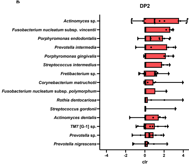
Supplementary Fig. S3 Top 15 bacterial taxa based on clr-transformed abundance values. The taxa are ordered by mean values, with the whiskers represent the minimum and maximum values. The box spans from the first quartile to the third quartile, while the line inside the box represents the median. Group names are as shown in Fig. 1.
