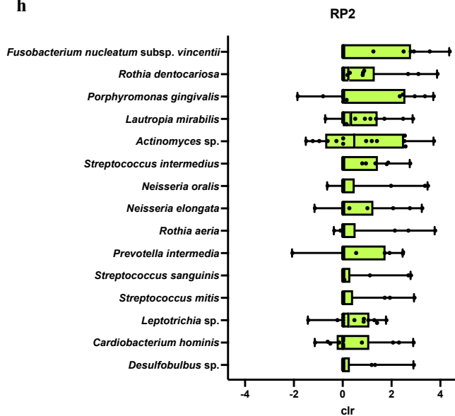
Supplementary Fig. S3 Top 15 bacterial taxa based on clr-transformed abundance values. The taxa are ordered by mean values, with the whiskers represent the minimum and maximum values. The box spans from the first quartile to the third quartile, while the line inside the box represents the median. Group names are as shown in Fig. 1.
