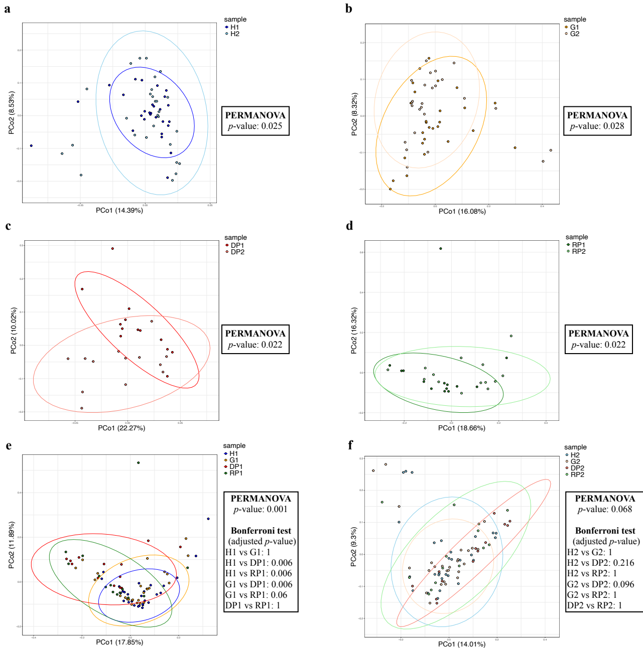
Supplementary Fig. S5 PCoA and PERMANOVA using Bray-Curtis distance based on the functional gene abundance from NCBI nr. Light colors indicate post-treatment samples for each group, contrasting with the darker colors for pre-treatment samples. The plots show each sample, and the ellipses indicate 95% confidence intervals. Group names are as indicated in Fig 1. (a-d) PCoA and PERMANOVA show longitudinal functional changes pre- and post-treatment using Bray-Curtis distance for the H, G, DP, and RP groups, respectively. (e, f) Multi-group comparisons between groups pre- and post-treatment using PCoA and PERMANOVA based on functional gene abundance.
