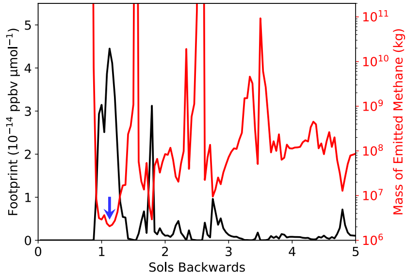
Fig. S7. An example time series of footprint magnitude for Spike 1 at the center of the “E8” region in supplementary ref. 2 (4°S, 144°E). The emission site is about 390 km away from the Curiosity rover. The black curve shows the STILT footprint versus time backwards with respect to the time of detection. The zero footprint within the first twenty hours means that any emission that takes place at this emission site less than twenty hours before the detection will not reach the detection site at Curiosity . The red curve shows the mass of emitted methane that can give rise to the methane signal, assuming methane is instantaneously emitted. The blue arrow indicates the moment of maximum influence of the emission site on the methane signal, which manifests itself as the smallest emitted methane abundance. To produce Spike 1, this emission site has to emit at least 2 \times 10^6 kilograms of methane, which is equivalent to 0.22 ppbv global mean methane concentration. This requires that the emission occurred at the exact moment when the emission site had the maximum influence on the detection, which is almost impossible. If the emission occurred at a random time within five sols before the detection, this figure shows that in general 10^7 to 10^8 kilograms of methane needs to be emitted. The emitted mass for the “E8” region found in supplementary ref. 2 is 1.17 \times 10^6 to 2.74 \times 10^6 kilograms, which is about the same as the lower limit estimated in this study.
