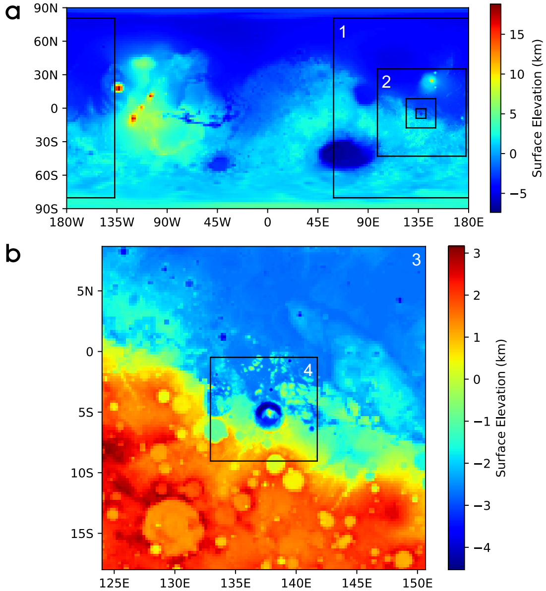
Fig. S1. MarsWRF domains on the four nesting levels. (a) Level 1, with a horizontal resolution of 2^\circ \times 2^\circ or \sim 118 \text{ km} \times \sim 118 \text{ km} , and level 2, 0.67^\circ \times 0.67^\circ or \sim 39 \text{ km} \times \sim 39 \text{ km} . (b) Level 3, 0.222^\circ \times 0.222^\circ or 13.1 \text{ km} \times 13.1 \text{ km} , and level 4, 0.74^\circ \times 0.74^\circ or 4.4 \text{ km} \times 4.4 \text{ km} . Colors show surface elevation in the corresponding horizontal resolutions of the four nesting levels.
