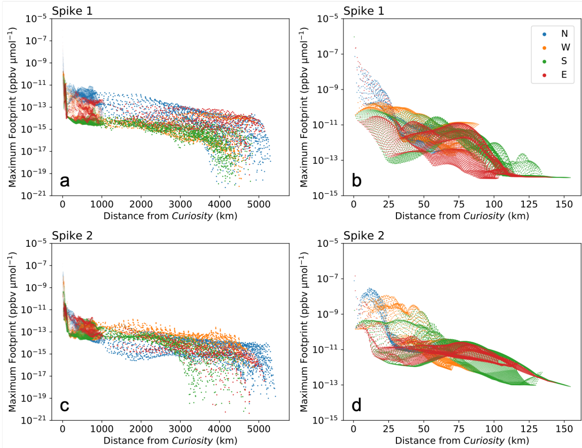
Fig. S8. Decay of STILT footprint with distance. Shown is the maximum STILT footprint ( (a) and (b) for Spike 1 and (c) and (d) for Spike 2 at every putative emission site around the detector versus the distance between the emission site and the detector. (a) and (c) show all the emission sites in Fig. 3(c). (b) and (d) only show emission sites within and in the vicinity of Gale crater. Blue dots indicate emission sites in the northern quadrant, yellow dots, in the western quadrant, green dots, in the southern quadrant, and red dots, in the eastern quadrant. The drop of footprint magnitude at long distances ( > 3000 km) in (a) and (c) is due to an insufficient number of particles that reach these distant places in the STILT simulations. It is found that the maximum footprint decays rapidly with distance while within Gale crater. Outside Gale crater, the decay is slower. This figure demonstrates of the necessity of modeling atmospheric dispersion when one wants to build a linkage between emission fluxes and methane signals, because the linkage strongly depends on the distance between an emission site and the detector.
