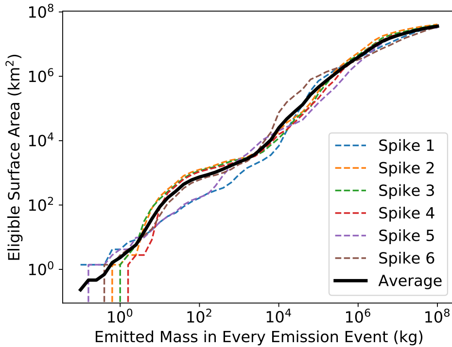
Fig. S10. The maximum area of the regions where different amounts of methane emission
