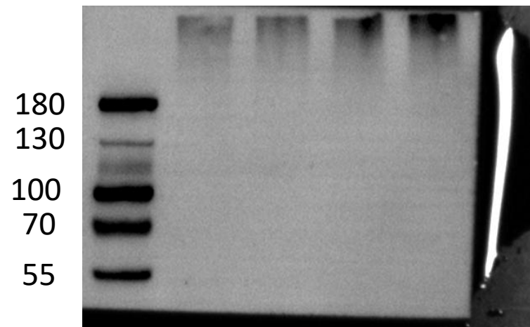
SHIP1 250kDa
