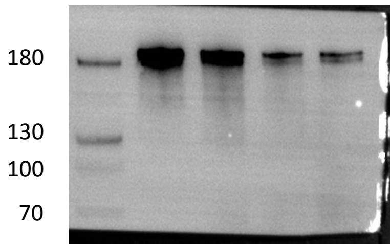
Nephrin 180kDa
