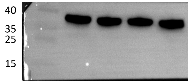
GAPDH 36kDa
