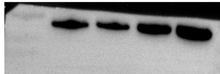
GAPDH 36kDa
