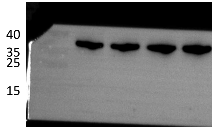
GAPDH 36kDa
