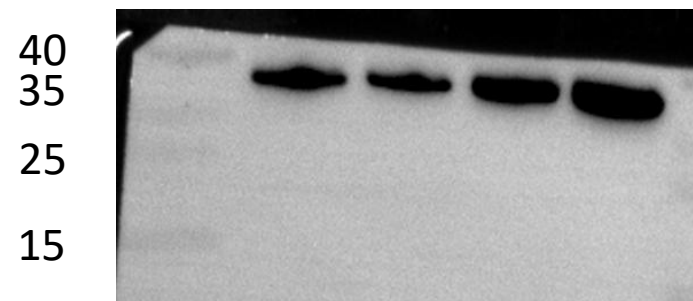
GAPDH 36kDa
