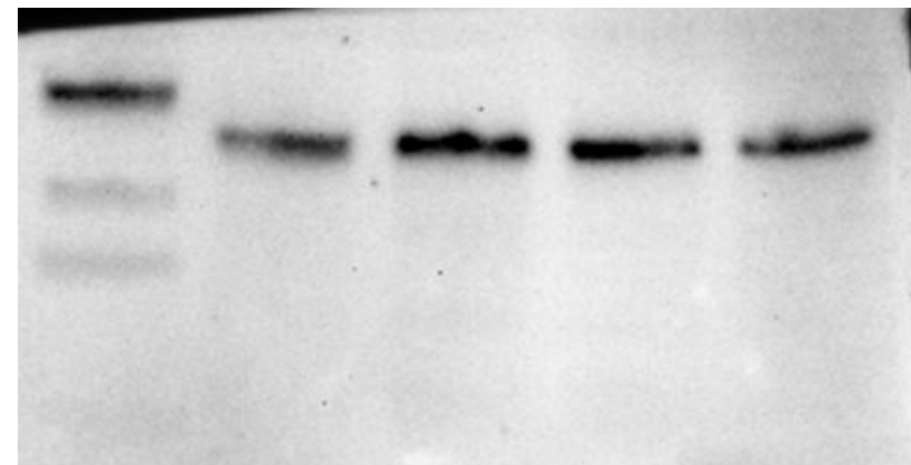
GAPDH 36kDa
