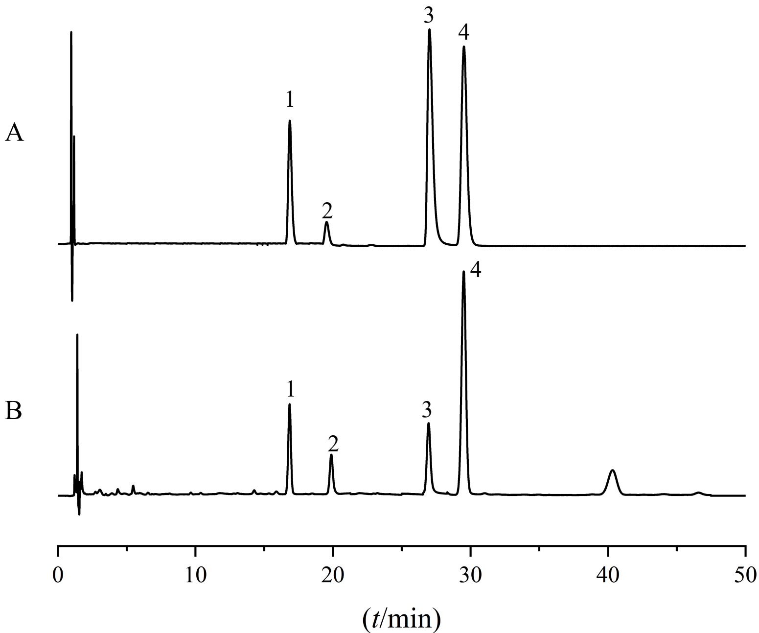
Fig. S8 UPLC chromatogram of mixing reference solutions (1. lasiodonin, 2. rosthosin A, 3. rosmarinic acid, 4. oridonin) and the I. rubescens samples of control group
