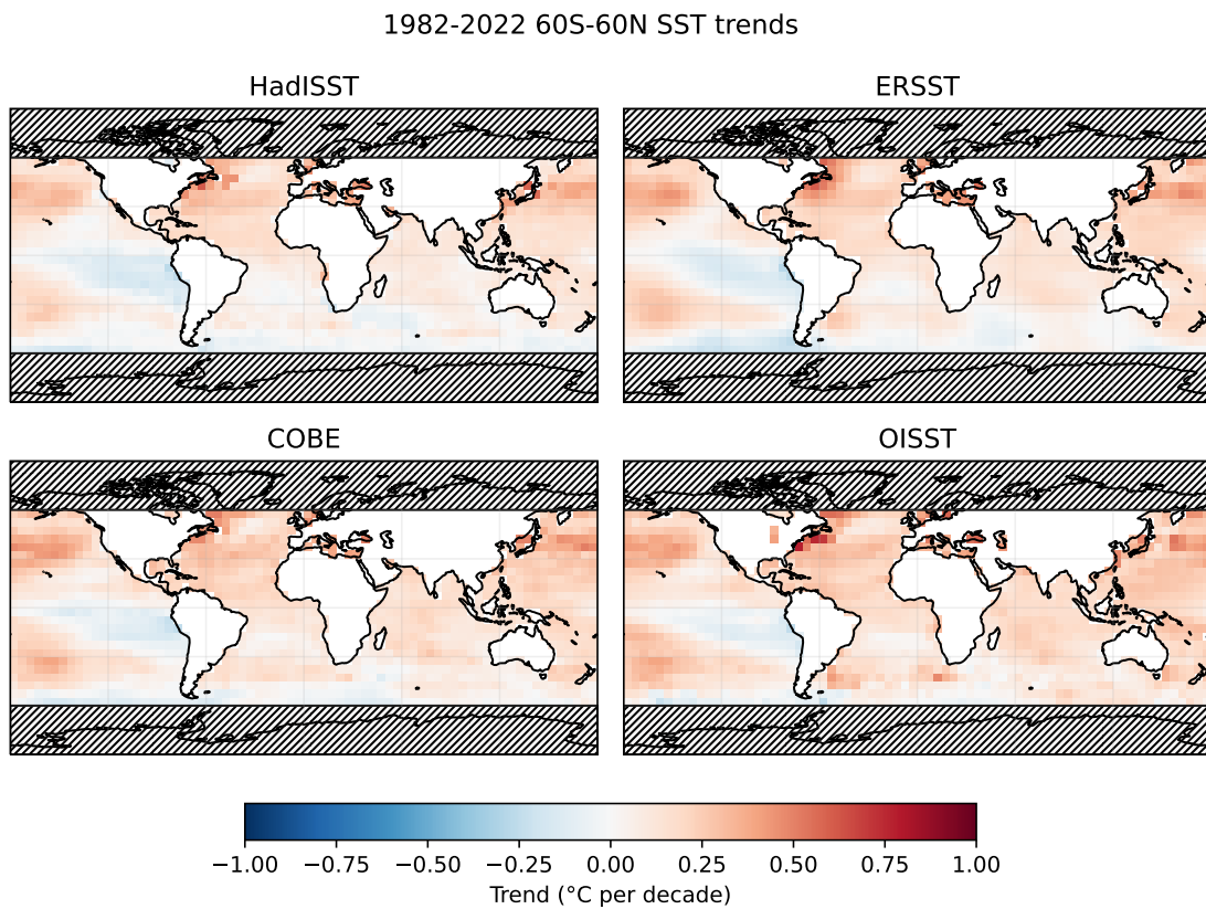
Figure S 1: 1982-2022 SST trends in HadISST1, ERSSTv5, COBE2, and OISSTv2.1.
