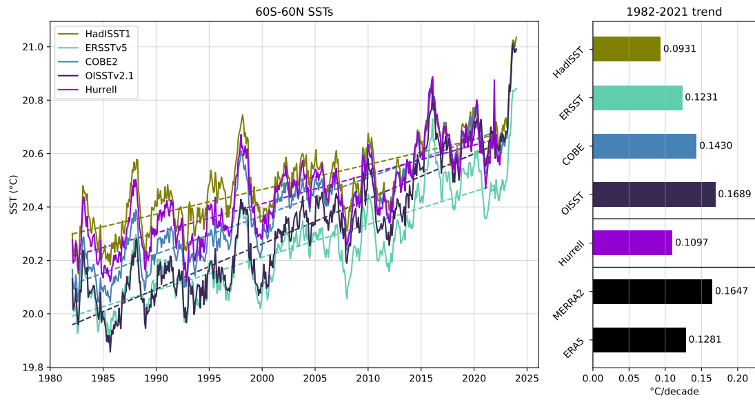
Figure S 4: Similar to Figure 1 in the main text, but including the Hurrell SSTs, shown in purple, and considering trends during the period 1982-2021 (since the year 2022 is not yet available for the Hurrell dataset).
