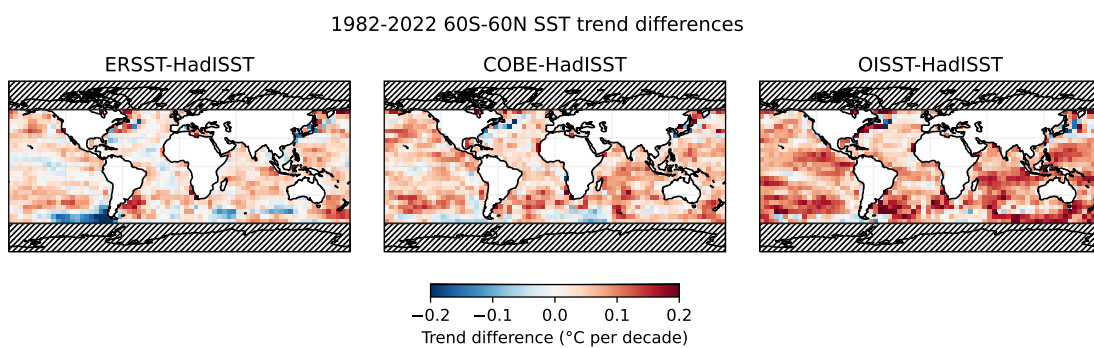
Figure S 2: Differences in 1982-2022 SST trends between ERSSTv5, COBE2, OISSTv2.1, and HadISST1.
