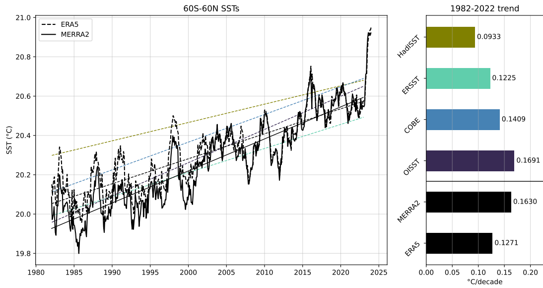
Figure S 3: Similar to Figure 1 in the main text, but including the timeseries and trendlines of MERRA2 and ERA5, and the trendlines from the datasets depicted in Figure 1 shown as dashed colored lines.
