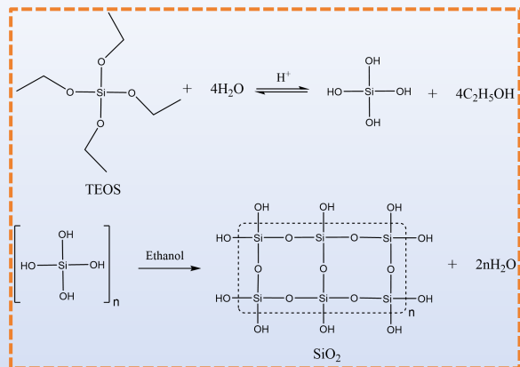
SiO 2 sol synthesis process
