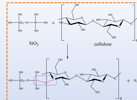
Synthesis path of SiO 2 and cellulose
