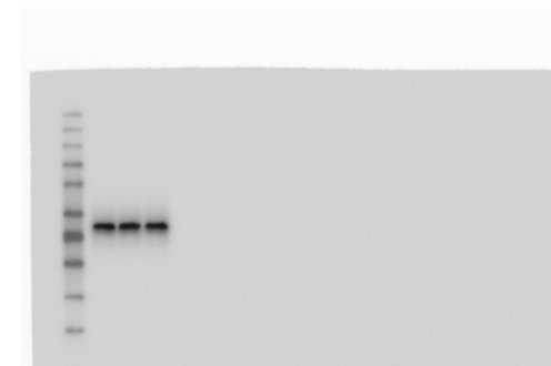
\beta -actin
