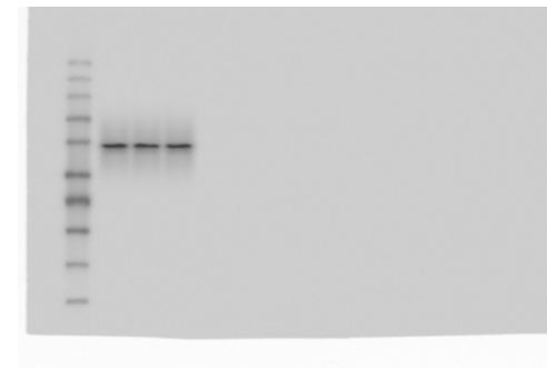
Frizzled-2
