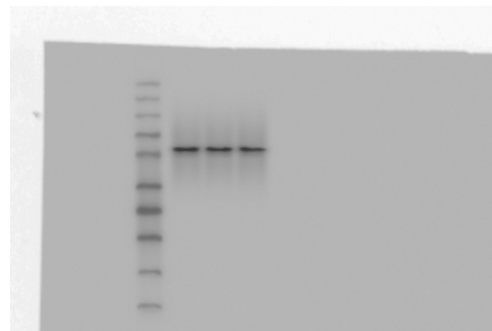
Frizzled-1
