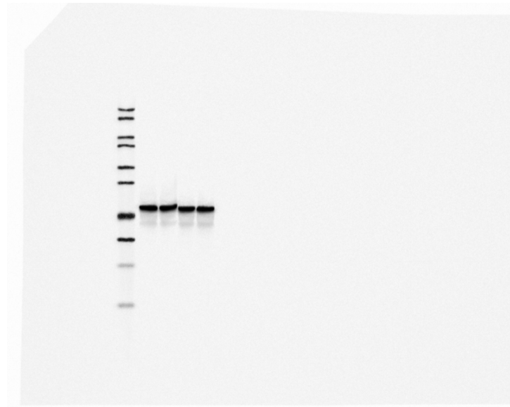
β-actin
