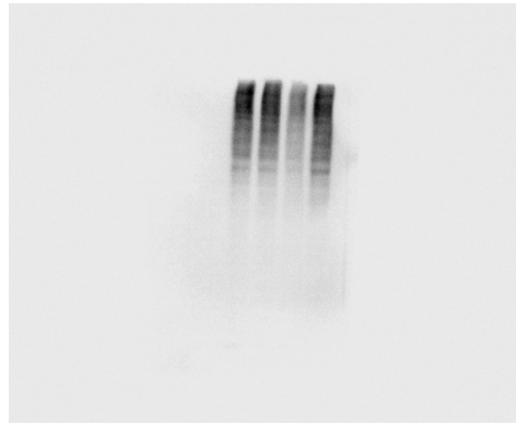
IP-Axin1-IB-Ubiquitin
