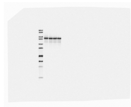
cytoplasm Dvl1
