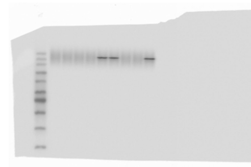
IP-HA IB-Flag
