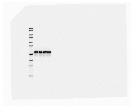
Na-K ATPase
