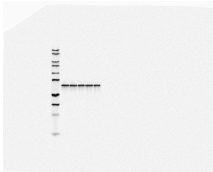
input-GSK3 \beta
