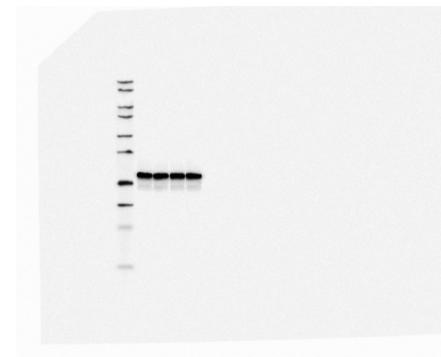
β-actin
