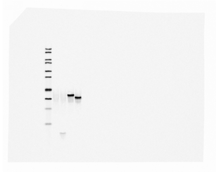
HA-Gβ2
