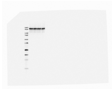
APC
