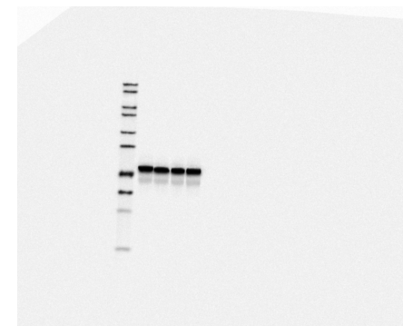
\beta -actin
