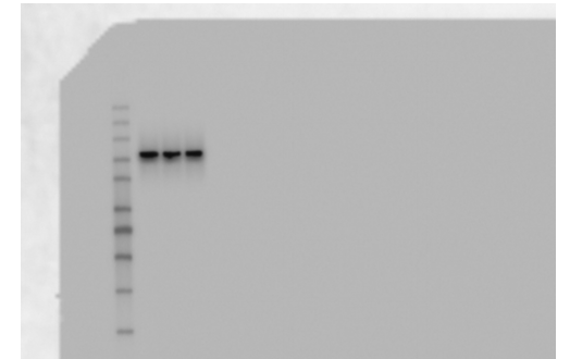
Na-K-ATPase
