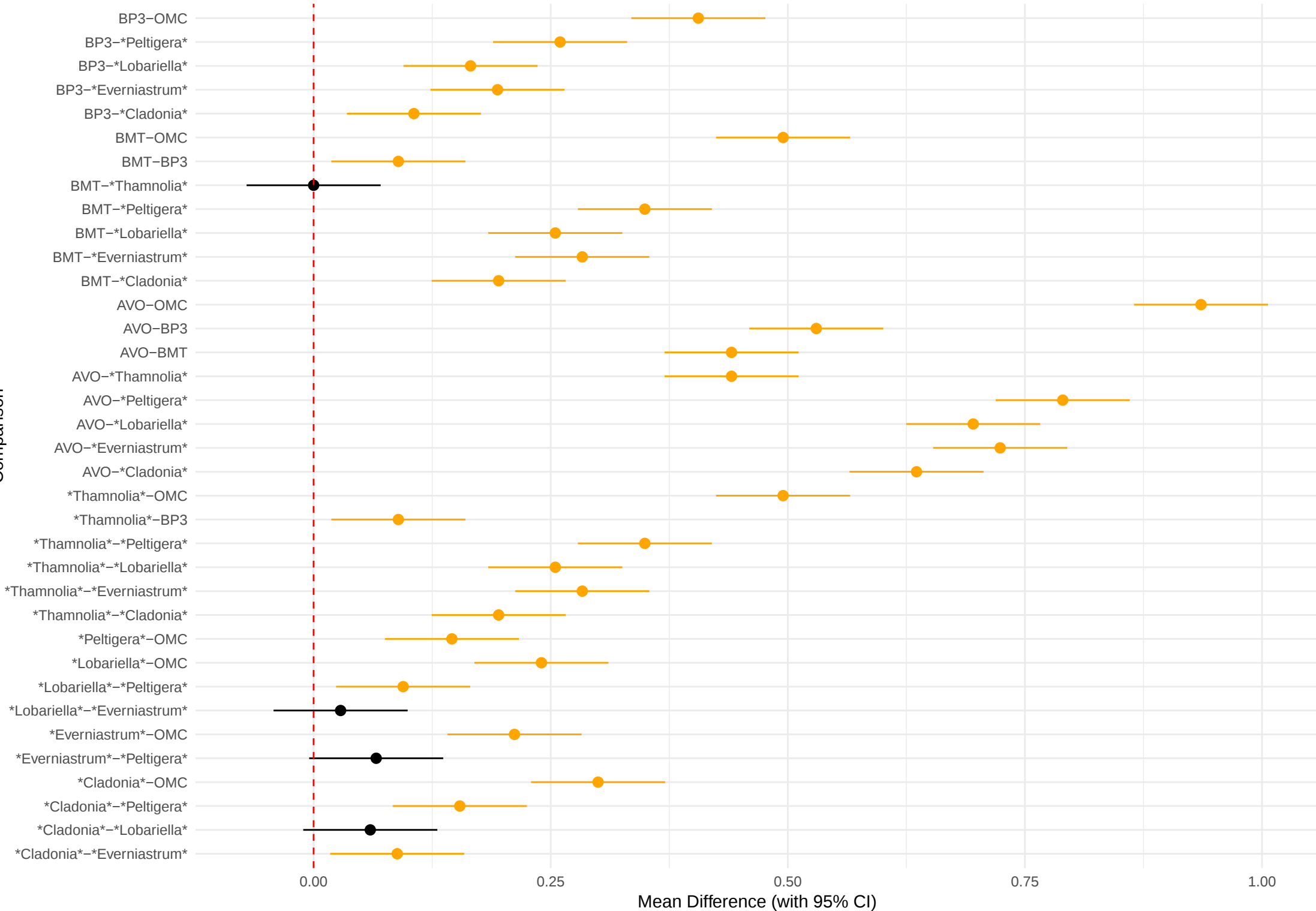
Tukey's HSD Post-Hoc Test Results – UVA-1 ratio
