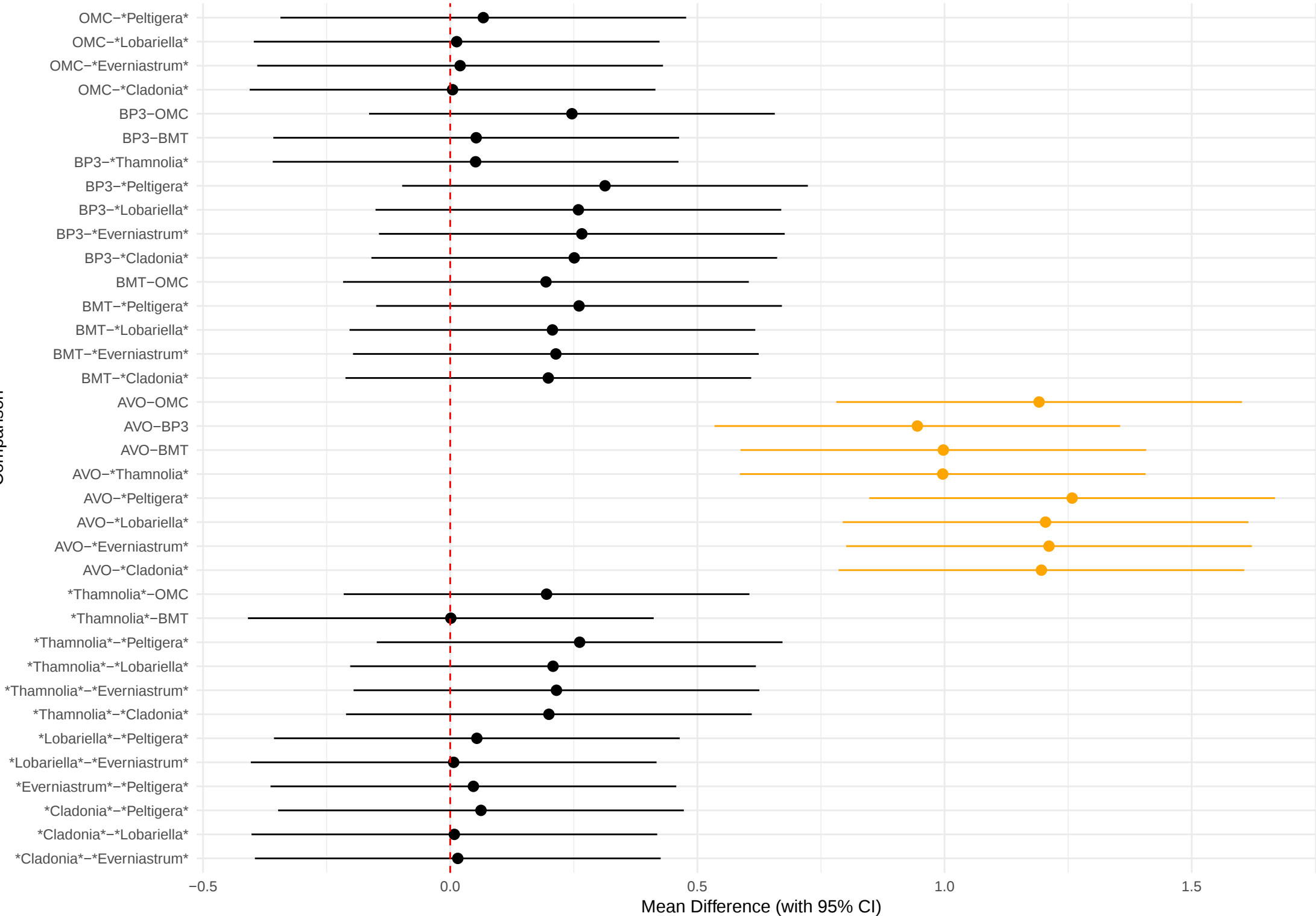
Tukey's HSD Post-Hoc Test Results – UVA/UVB ratio
