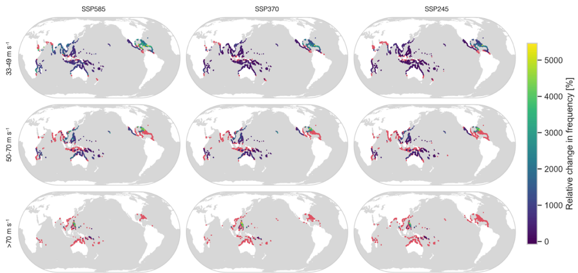
SM Figure 1: Relative change in frequency ECEarth
