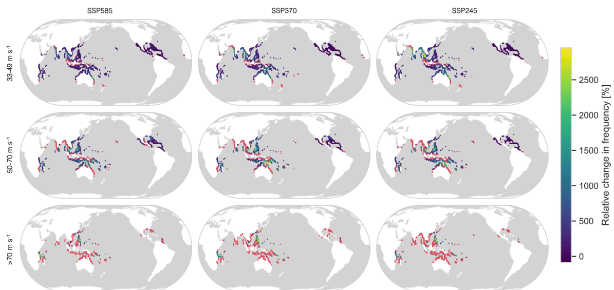
SM Figure 2: Relative change in frequency CESM2
