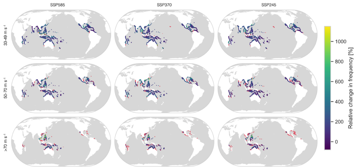
SM Figure 3: Relative change in frequency MIROC6
