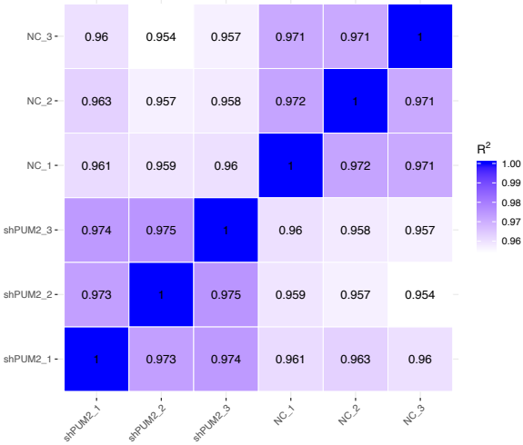
Pearson correlation between samples
