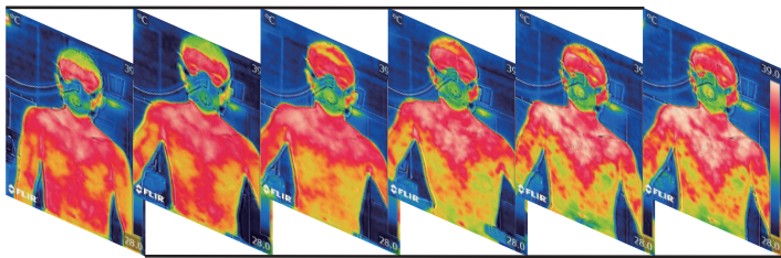
Temperature matrix
