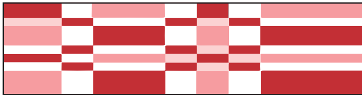
Entropy matrix
