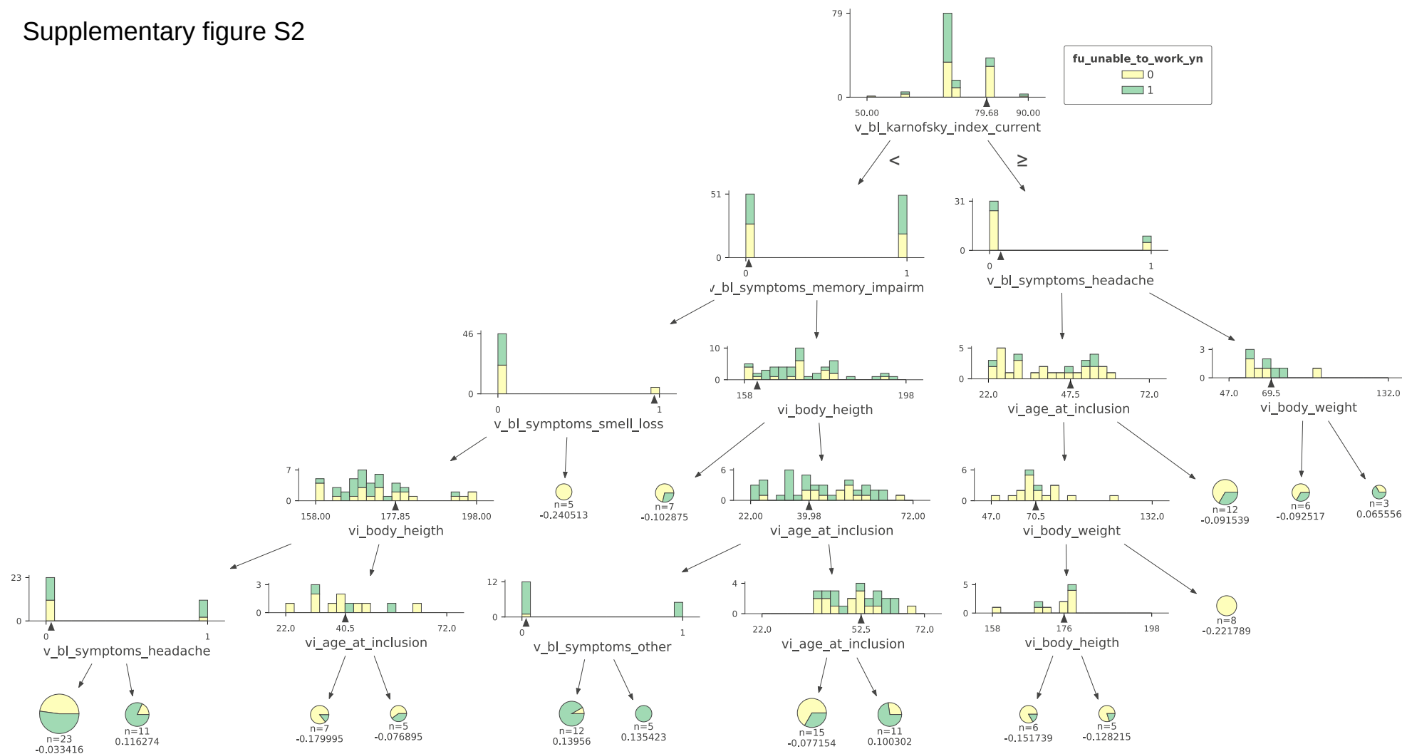
Supplementary figure S2. Exemplary decision tree of the TDFD-GB model. The model was trained with 300 trees. This figure depicts all levels of an exemplary decision tree.
