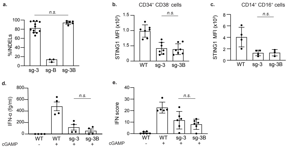
Supplementary Fig. 1 Efficient single guide RNA does not need to be combined to achieve high levels of gene editing. a. Percent INDELs for sgRNA-3 (n = 12), sgRNA-B (n = 3) and sgRNA-3 + sgRNA-B (sg-3B) (n = 6). FACS-based quantification of STING1 protein expression in b. HSPCs [WT (n = 7), sgRNA-3 treated (n = 7) and treated by sgRNA-3 + sgRNA-B (n = 7)] and in c. monocytes/macrophages after differentiation [day 15 (n = 4)]. d. Quantification of IFN- \alpha secretion in media and e. IFN score on day 15 of INDEL-GE -derive monocytes/macrophages, before (-) and after (+) cGAMP treatment. Data shown as mean \pm sem. Stats: Mann-Whitney test (panels a - e ).
