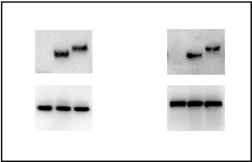
A2780/DDP/KD
