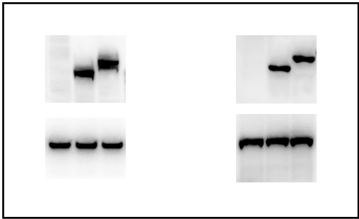
SKOV3/DDP/KD
