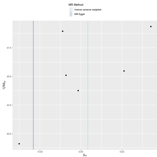
Supplementary Fig.5 Funnel plot of colorectal adenoma and cancer on the causality of diverticular disease.(a) Colorectal Adenoma;(b)CRC;(c)Proximal Colon Cancer;(d)Distal Colon Cancer;(e)Rectal Cancer;
