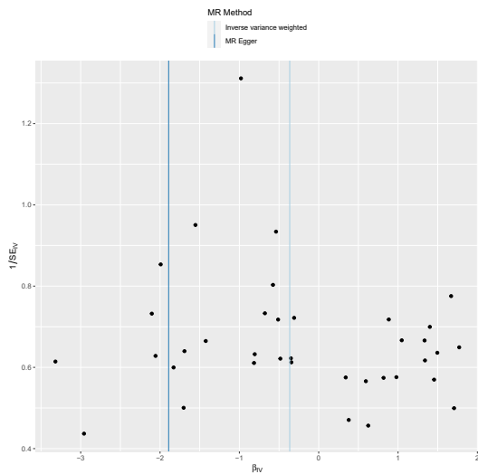
Supplementary Fig.2 Funnel plot of diverticular disease on the causality of colorectal adenoma and cancer.(a) Colorectal Adenoma;(b)CRC;(c)Proximal Colon Cancer;(d)Distal Colon Cancer;(e)Rectal Cancer;
