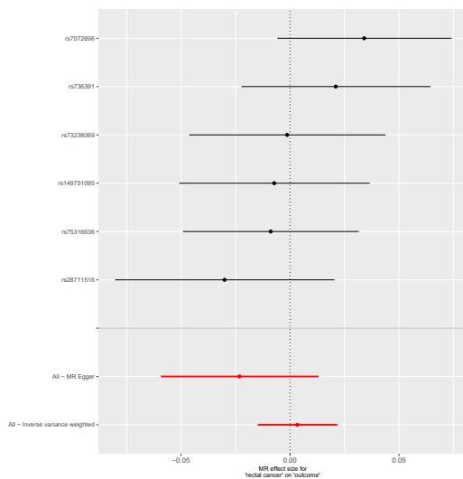
Supplementary Fig.6 Forest plot of colorectal adenoma and cancer on the causality of diverticular disease.(a) Colorectal Adenoma;(b)CRC;(c)Proximal Colon Cancer;(d)Distal Colon Cancer;(e)Rectal Cancer;
