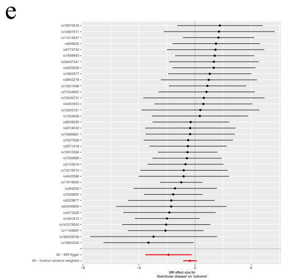
Supplementary Fig.3 Forest plot of diverticular disease on the causality of colorectal adenoma and cancer.(a) Colorectal Adenoma;(b)CRC;(c)Proximal Colon Cancer;(d)Distal Colon Cancer;(e)Rectal Cancer;
