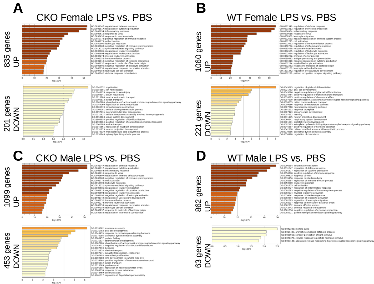
Figure S4: Bar graph of enriched terms across input gene lists, colored by p-values. P-values are also shown on the X-axis.
