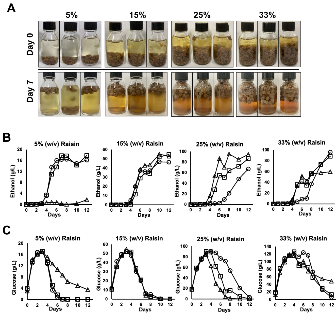
Supplementary Figure 4. Effects of raisin contents on ethanol production and glucose consumption. (A) Images of raisin water. Ethanol (B) and glucose (C) concentrations ( n = 3 indicated by circles, squares, and triangles).
