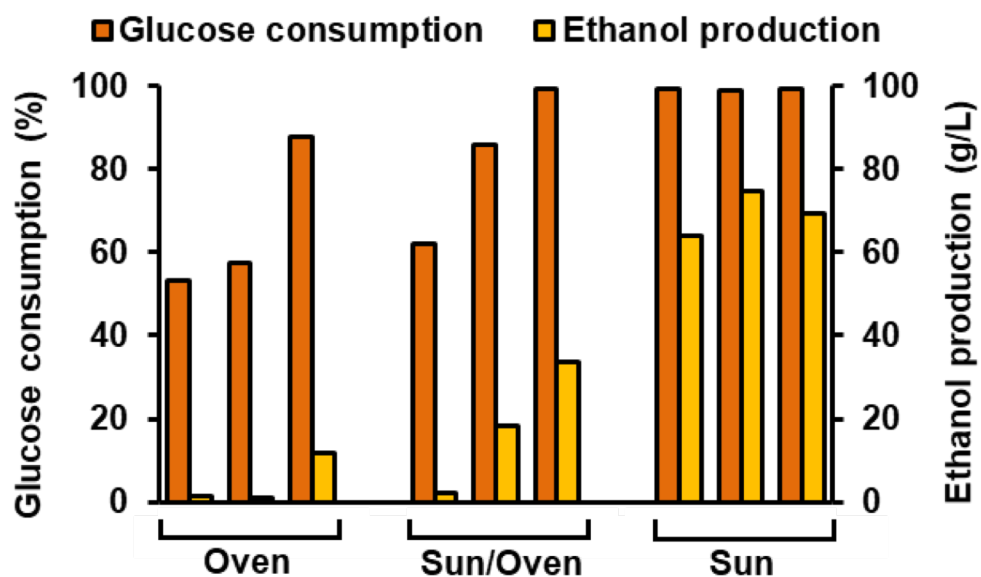
Supplementary Figure 11. Ethanol production and glucose consumption of raisin water made from laboratory-made raisins.
