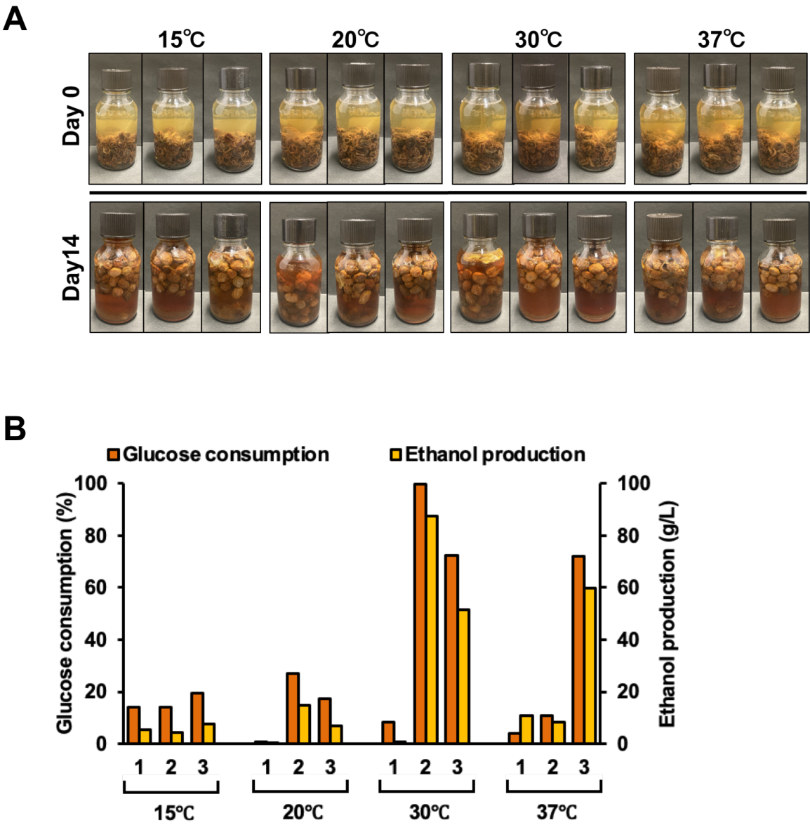
Supplementary Figure 5. Effects of incubation temperatures on ethanol production. (A) Images of the raisin water samples. (B) Ethanol and glucose concentrations on Day 14.
