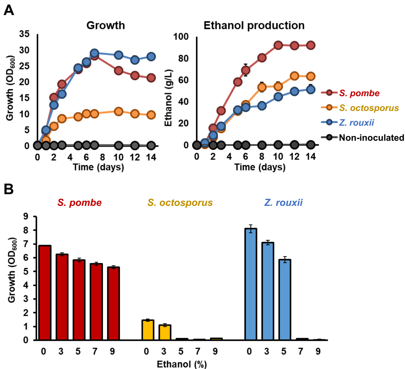
Supplementary Figure 3. Ethanol production and ethanol tolerance of raisin-isolated yeasts. (A) Growth and ethanol production by S. pombe , S. octosporus , and Z. rouxii isolated from the water squeezed from raisins (n = 3, mean \pm SD). (B) Effects of spiked ethanol on the growth of the isolates (n = 3, mean \pm SD). OD 600 was measured on Day 7.
