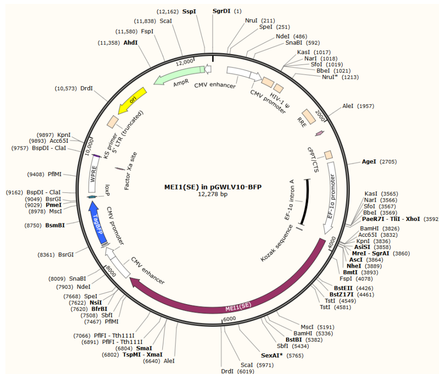
Supplementary Figure S4 Plasmid profile of MEI1 (SE) in pGWL10-BFP
