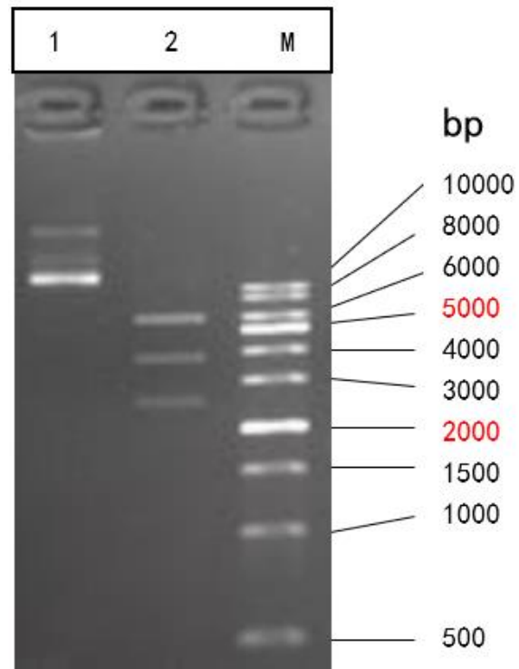
Supplementary Figure S3 MEI1 (SE) in pGWL V10-BFP was detected by agarose gel electrophoresis
