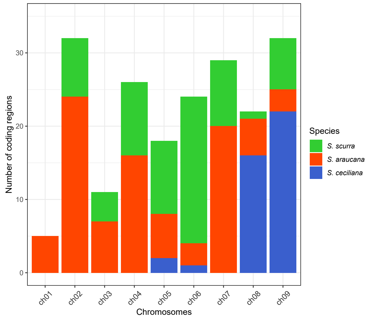
B) Divergence in Allopatry
