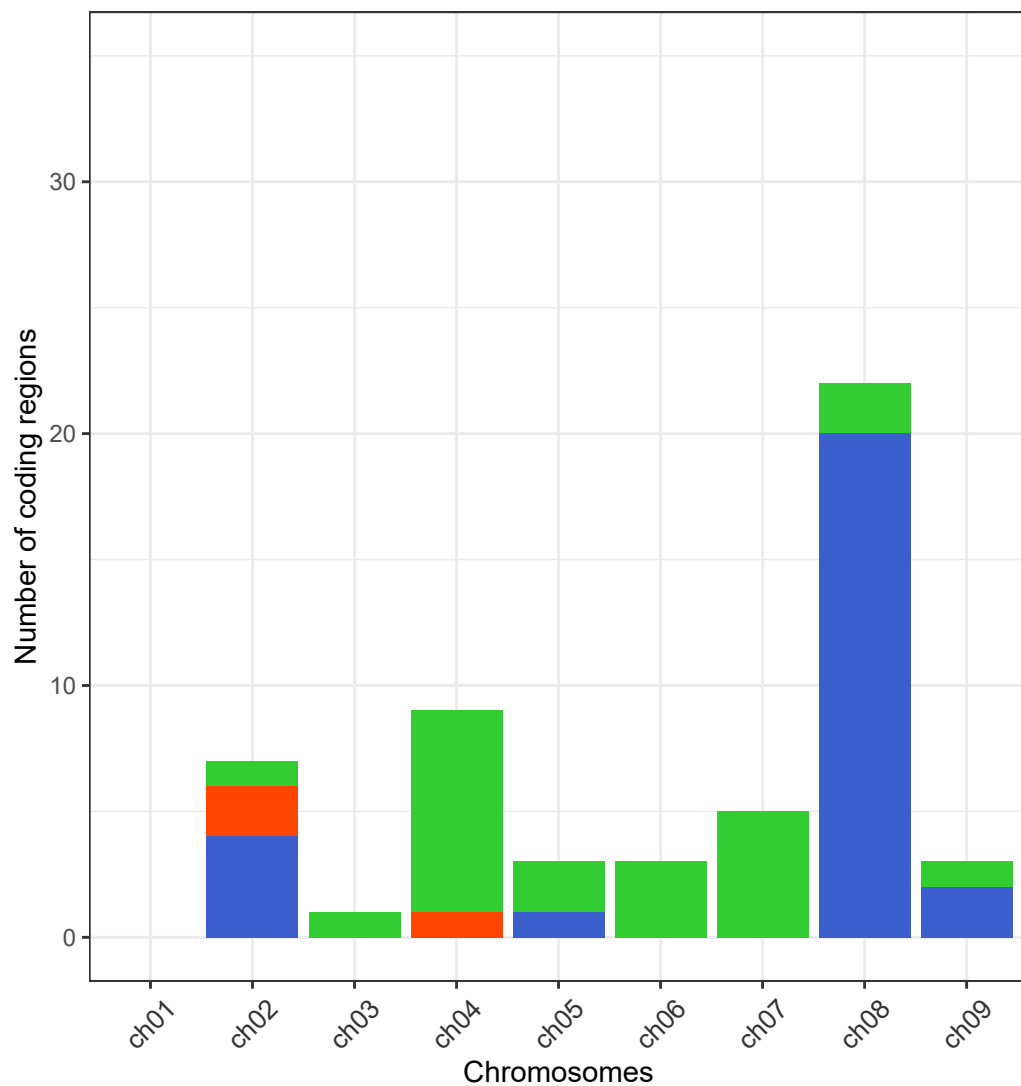
A) Divergence with gene flow
