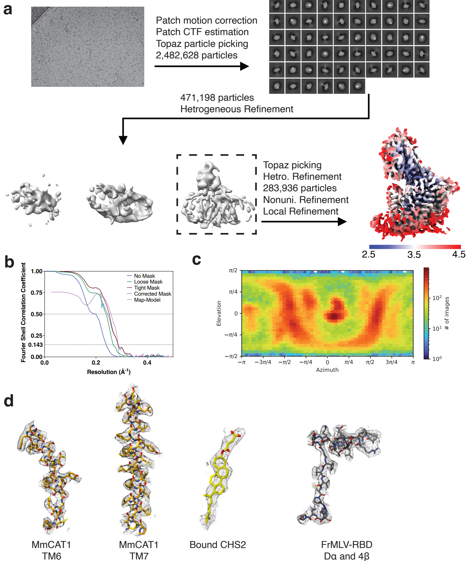
Extended Data Figure 7. Structure determination of the apo MmCAT1:FrMLV-RBD complex. (a) Flow chart for determining the structure of the substrate free MmCAT1:FrMLV-RBD complex. (b) Fourier shell correlation coefficient for cryo-EM map reconstruction and model refinement. (c) Particle orientation distribution for cryo-EM map reconstruction. (d) Representative density for MmCAT1, FrMLV-RBD, and bound cholesterol hemisuccinate (CHS).
