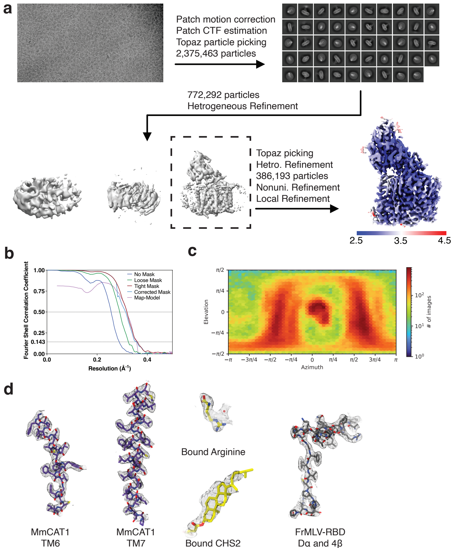
Extended Data Figure 2. Structure determination of the Arginine bound MmCAT1:-FrMLV-RBD complex. (a) Flow chart for determining the structure of the Arginine bound MmCAT1:FrMLV-RBD complex. (b) Fourier shell correlation coefficient for cryo-EM map reconstruction and model refinement. (c) Particle orientation distribution for cryo-EM map reconstruction. (d) Representative density for MmCAT1, FrMLV-RBD, and bound arginine and cholesterol hemisuccinate (CHS).
