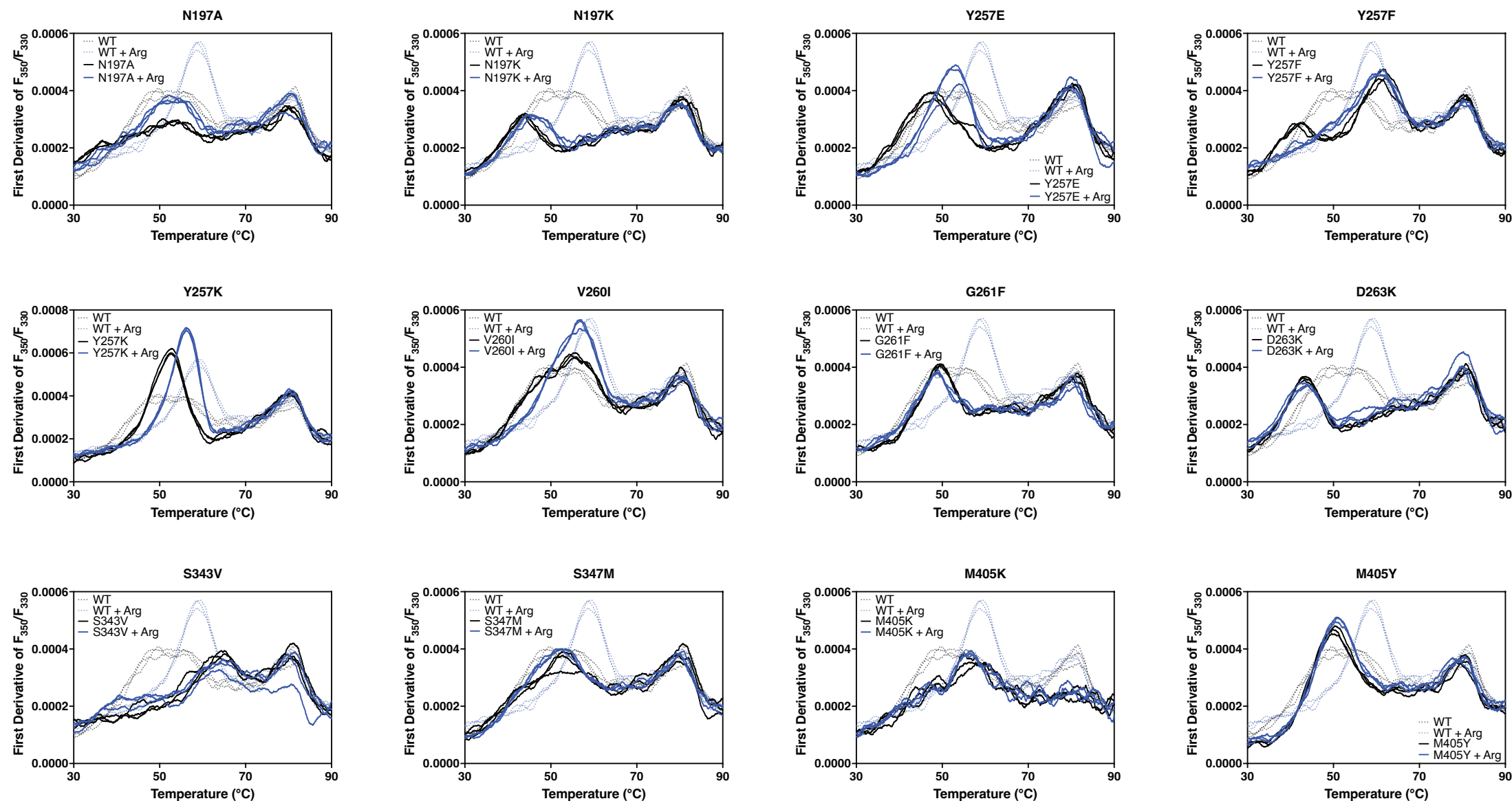
Extended Data Figure 4. ThermoStability of MmCAT1 mutants with and without arginine. NanoDSF for each mutant, purified in LMNG/CHS, with and without ligand. Individual experiments are shown for each experiment of technical replicates (N=3) as solid lines and dotted lines for mutants and wild type protein, respectively.
