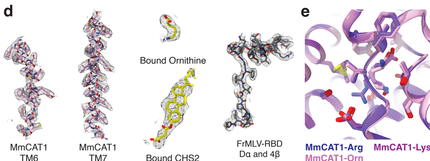
Extended Data Figure 6. Structure determination of the ornithine-bound MmCAT1:FrMLV-RBD complex. (a) Flow chart for determining the structure of the ornithine-bound MmCAT1:FrMLV-RBD complex. (b) Fourier shell correlation coefficient for cryo-EM map reconstruction and model refinement. (c) Particle orientation distribution for cryo-EM map reconstruction. (d) Representative density for MmCAT1, FrMLV-RBD, and bound ornithine and cholesterol hemisuccinate (CHS). (e) Overlay of MmCAT1 substrate binding site bound to arginine, lysine, and ornithine.
