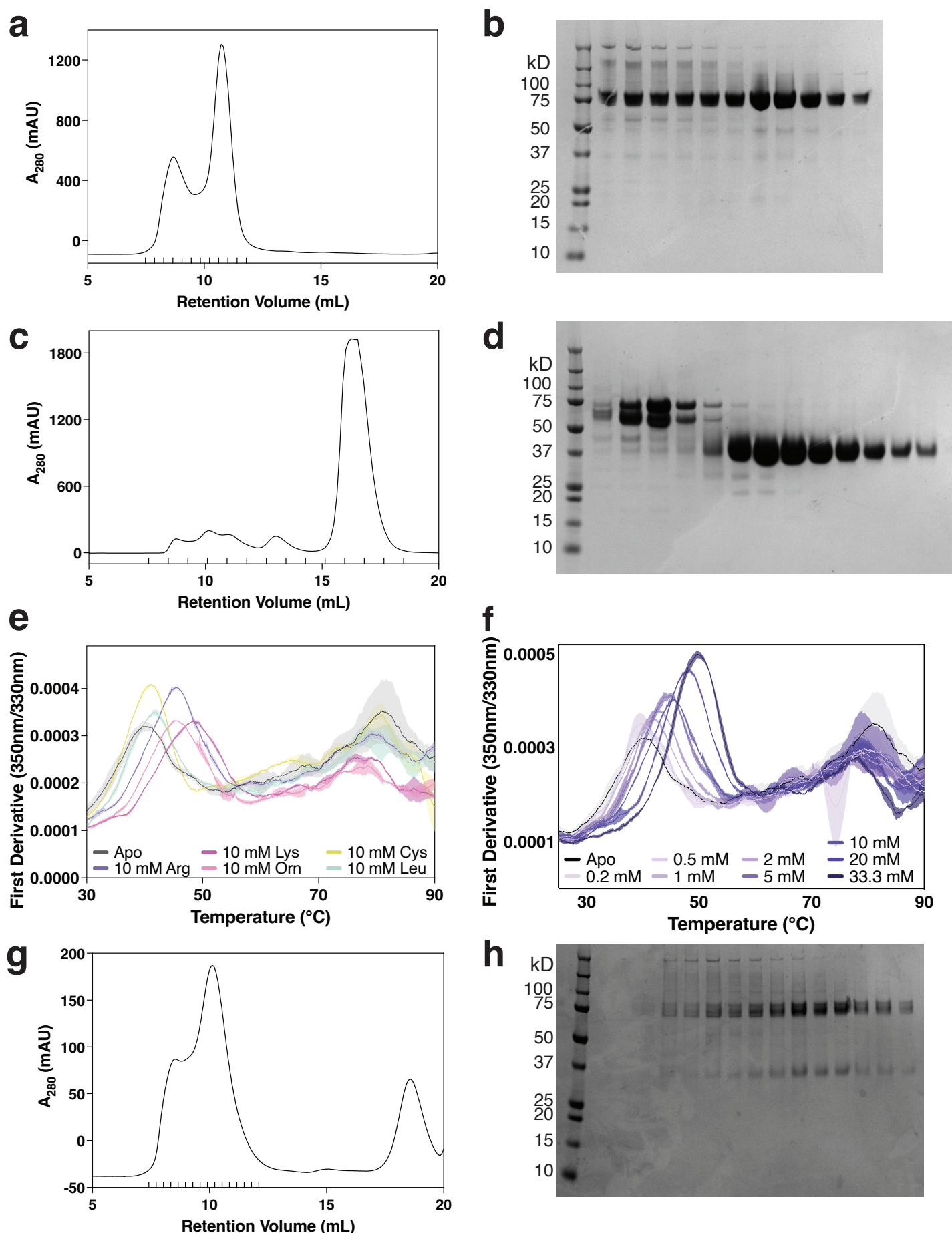
Extended Data Figure 1. Purification of MmCAT1, FrMLV-RBD, and MmCAT1:FrMLV-RBD complex. Purification of MmCAT1 by (a) preparative size-exclusion chromatography of MmCAT1 on a Superdex 200 Increase 10/300 GL column and (b) representative SDS-PAGE of MmCAT1 purification from 10 biological replicates. Purification of FrMLV-RBD by (c) preparative size-exclusion chromatography of MmCAT1 on a Superdex 200 Increase 10/300 GL column and (d) representative SDS-PAGE of MmCAT1 purification from 10 biological replicates. NanoDSF of MmCAT1 with (e) various amino acids and (f) various concentrations of arginine. Purification of MmCAT1:FrMLV-RBD by (g) preparative size-exclusion chromatography of MmCAT1 on a Superdex 200 Increase 10/300 GL column and (h) representative SDS-PAGE of MmCAT1 purification from 10 biological replicates.
