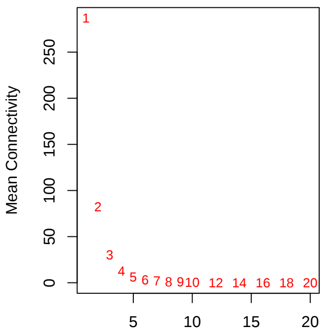
Mean connectivity
