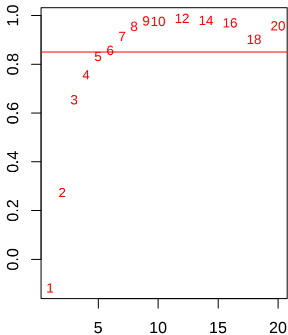
Scale independence
