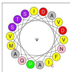
YP_001274308 ( M. smithii ) MIVPSAFASDAVDNQTVISSDEQIEISAV Hydrophobicity: 0.542
