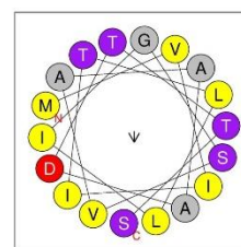
YP_448066 ( M. stadtmanae ) MVIITLLIGSVAAADTTS Hydrophobicity: 0.741
