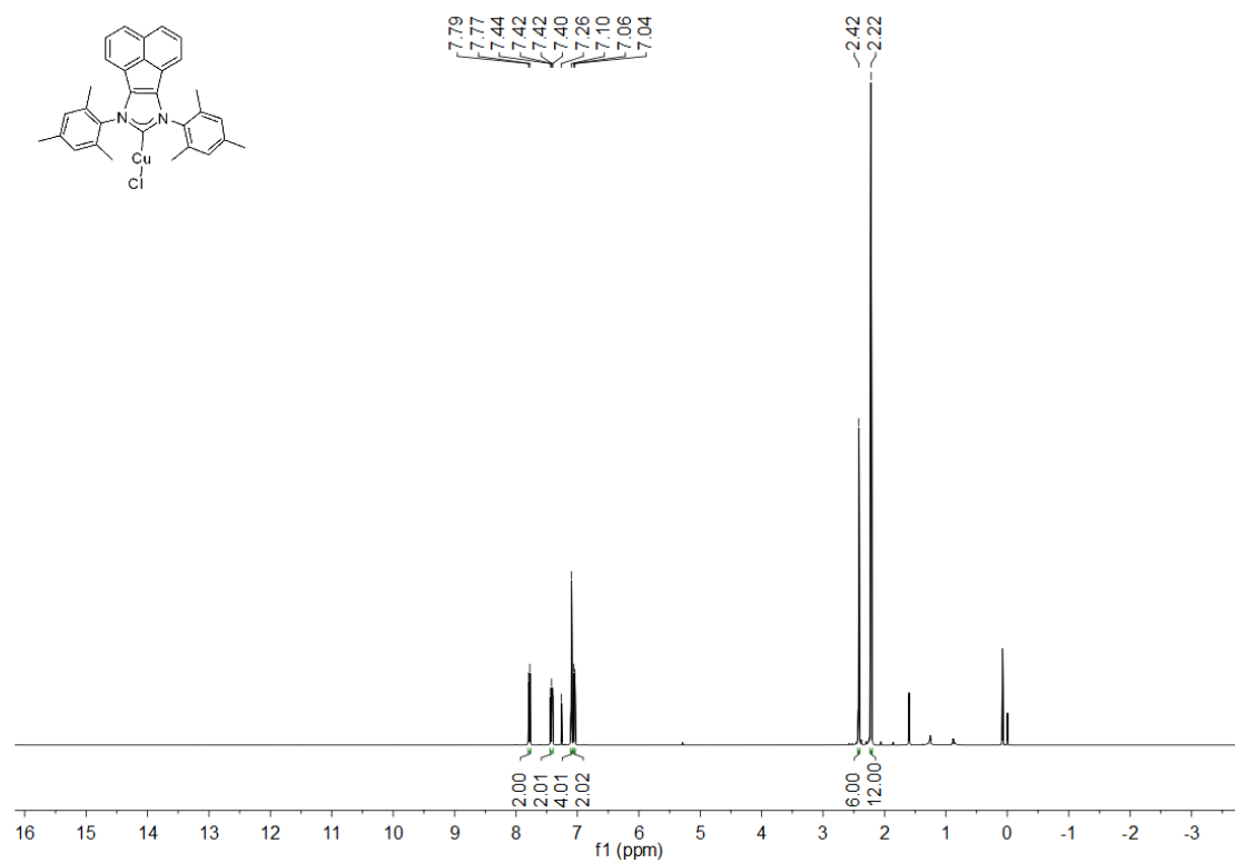
Figure S2. The NMR spectrum of Cu4
