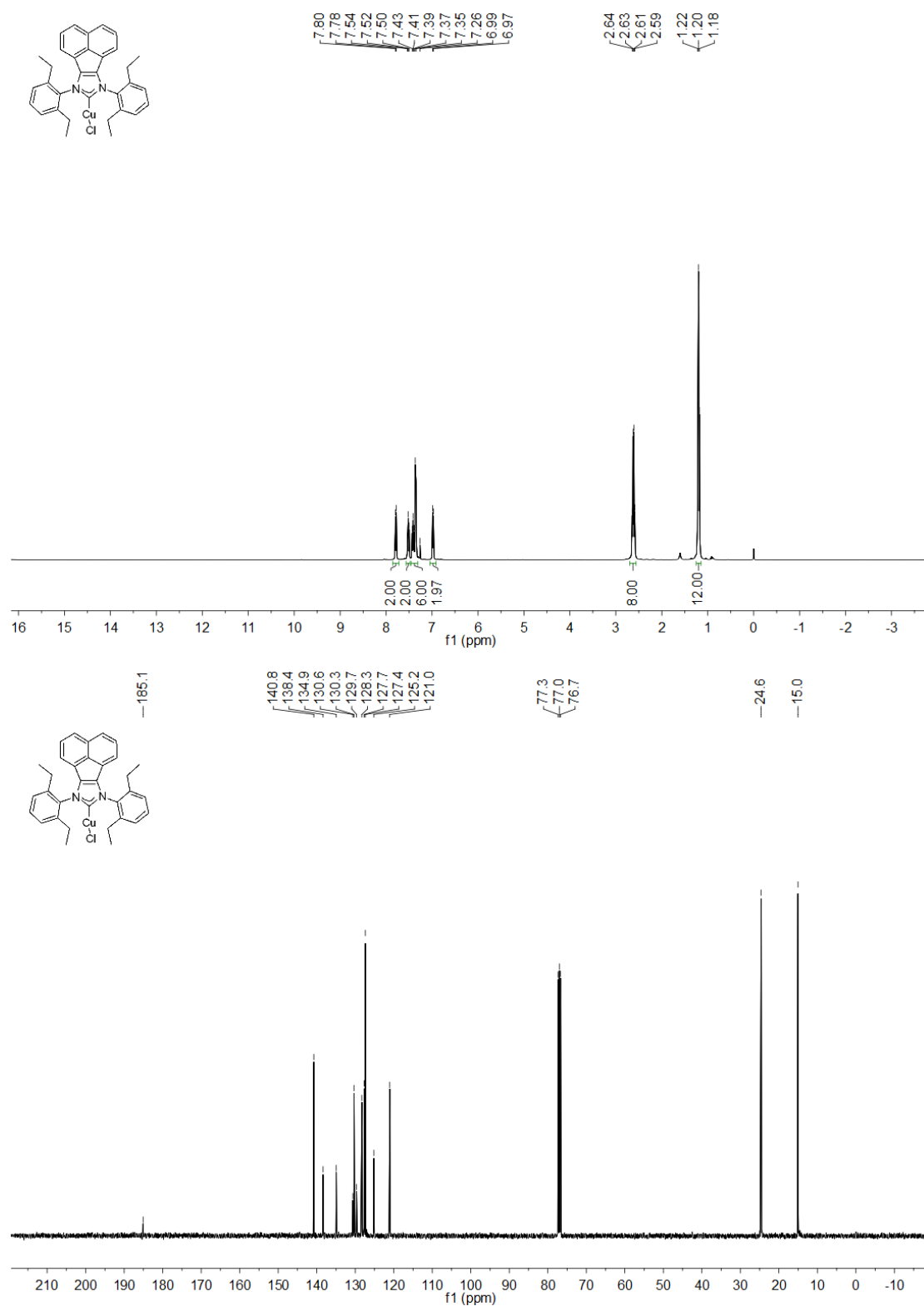
Figure S4. The NMR spectrum of Cu6
