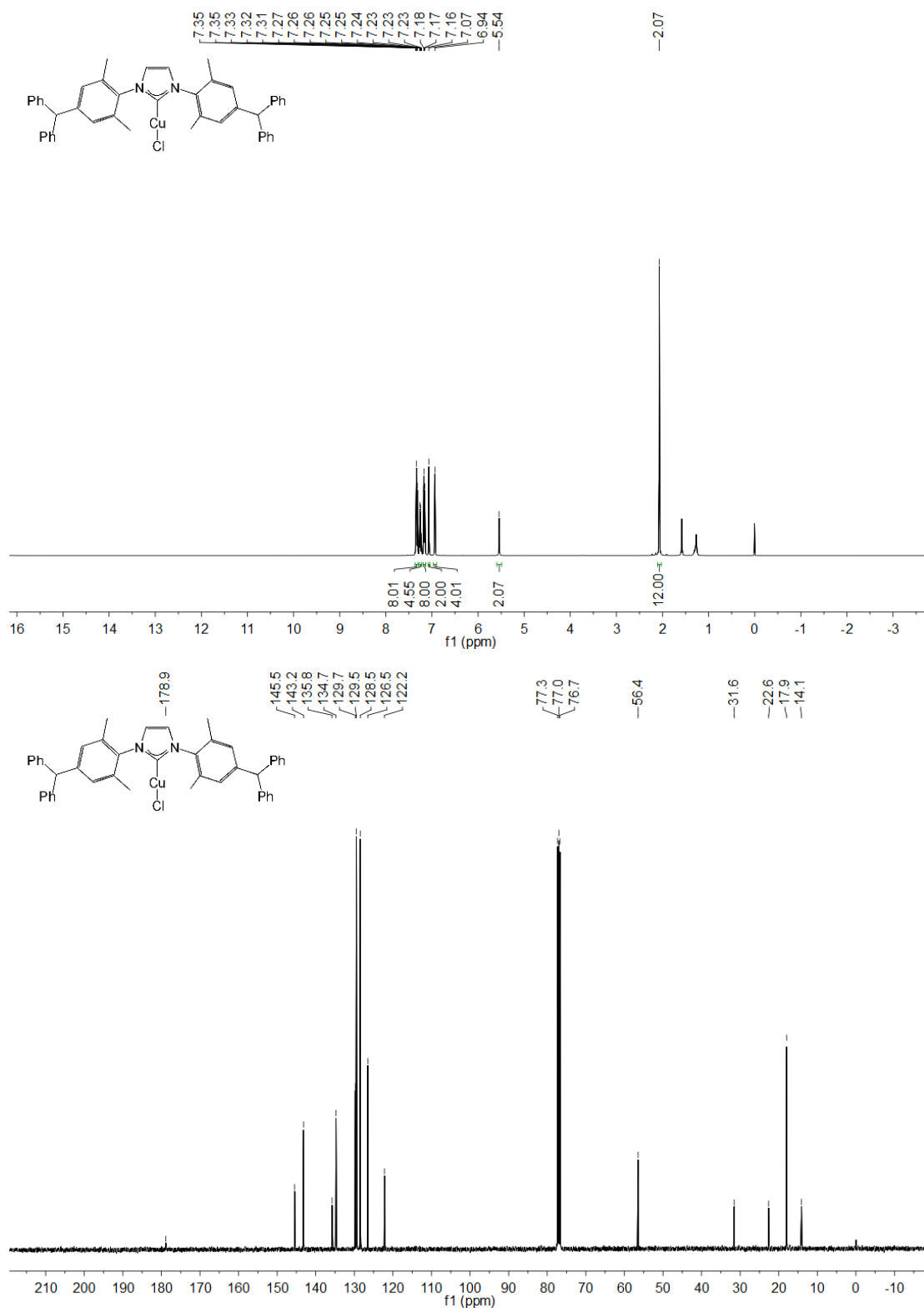
Figure S1. The NMR spectrum of Cu2
