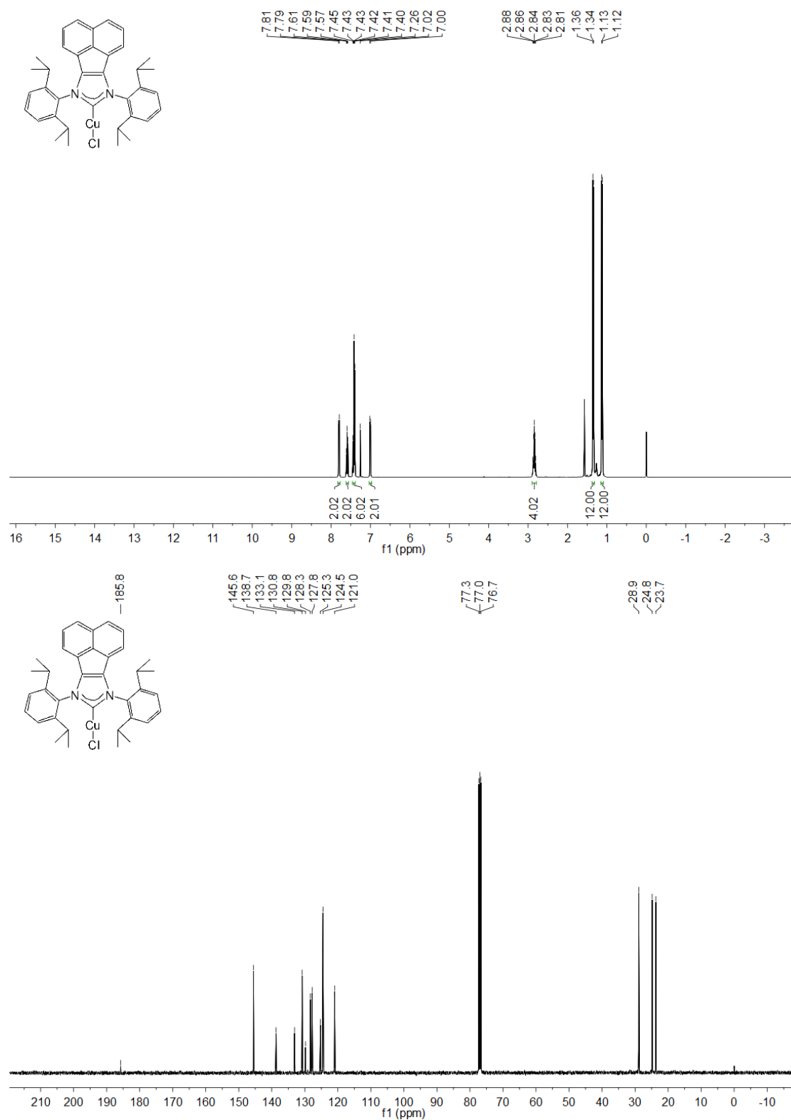
Figure S5. The NMR spectrum of Cu7
