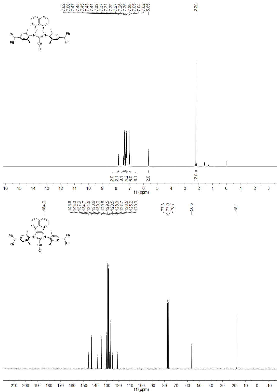
Figure S3. The NMR spectrum of Cu5
