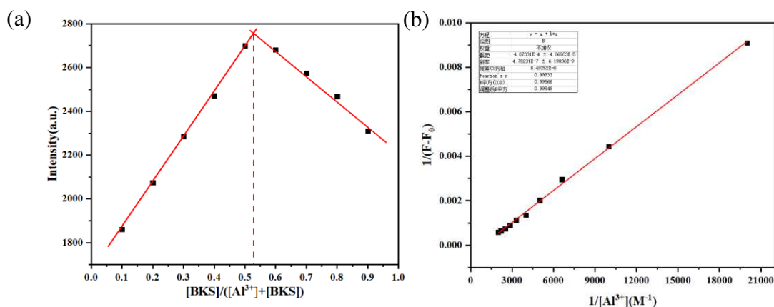
Fig.7 (a) Job's plot of probe BKS with \text{Al}^{3+} ; (b) Benesi-Hilbrand plot of probe BKS with \text{Al}^{3+} .
