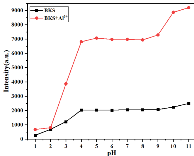
Fig.4 Scatter plot of fluorescence intensity at 545 nm with pH.
