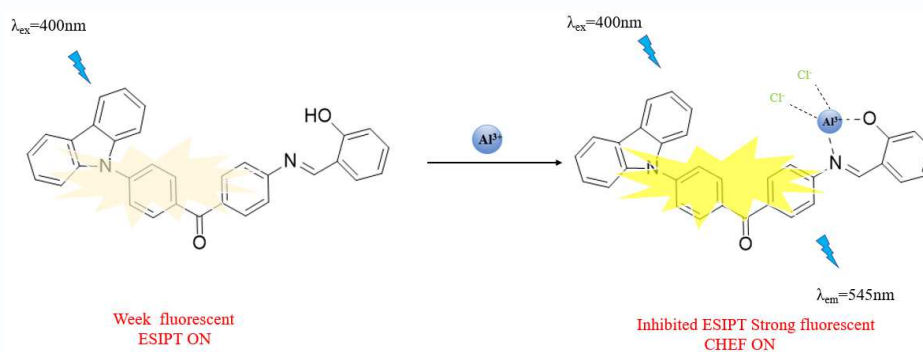
Fig. 2 (a) Fluorescence spectra of BKS probe (10 μM) upon addition of different metal ions (5.0 equiv.) in THF/H 2 O (v/v=1:4 HEPBS=10 mM, pH=7.40); (b) Fluorescence response of adding \text{Al}^{3+} to the solution containing BKS and various ions (black bars are the solution of BKS With various cations, red bars are the solution after adding \text{Al}^{3+} ); (c) visual fluorescence color changes of BKS probe (10 μM) in the presence of different metal ions under UV light at 365 nm.
