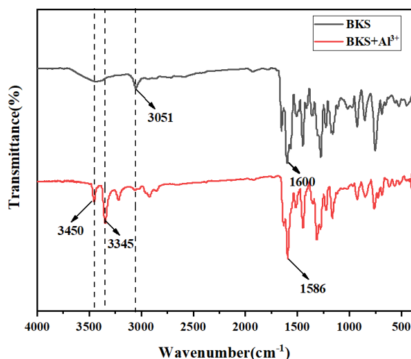
Fig.8 IR spectrum of probe BKS and probe BKS+Al 3+ .
