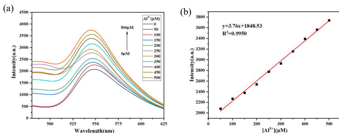
Fig. 3 (a) Fluorescence spectra of BKS at 545 nm with various concentrations of \text{Al}^{3+} (0-500 \mu\text{M} ); (b) The linear relationship of the fluorescence intensity of BKS- \text{Al}^{3+} at 545 nm versus the concentration of \text{Al}^{3+} .
