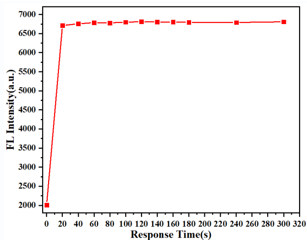
Fig.5 Response time spectra of fluorescent probe BKS to \text{Al}^{3+}
