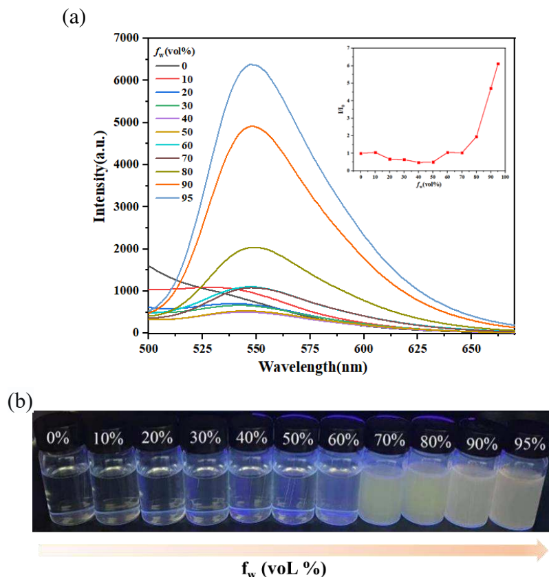
Fig.1 (a) Fluorescence emission spectra of BKS probe in THF/H 2 O solutions ( f_w=0 -95%) at 400 nm of excitation wavelength. Inset: Plots of FL intensity of BKS probe versus f_w in THF/H 2 O mixtures; (b) the photos of BKS probe (10 \mu M) under 365 nm UV light in different THF/H 2 O mixed solution.
