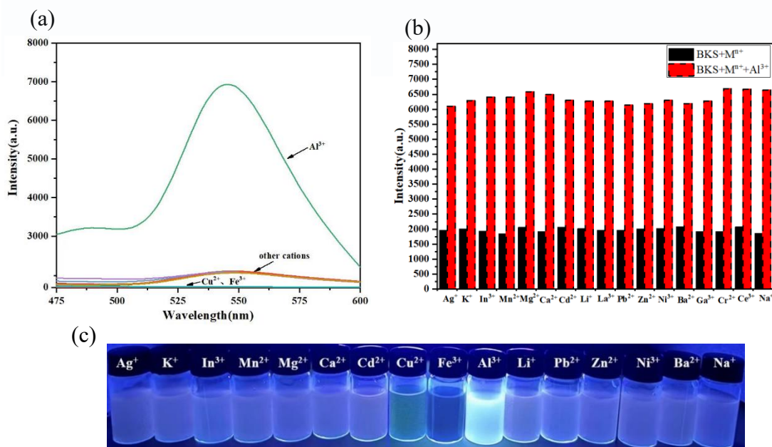
Fig. 2 (a) Fluorescence spectra of BKS probe (10 μM) upon addition of different metal ions (5.0 equiv.) in THF/H 2 O (v/v=1:4 HEPBS=10 mM, pH=7.40); (b) Fluorescence response of adding \text{Al}^{3+} to the solution containing BKS and various ions (black bars are the solution of BKS With various cations, red bars are the solution after adding \text{Al}^{3+} ); (c) visual fluorescence color changes of BKS probe (10 μM) in the presence of different metal ions under UV light at 365 nm.
